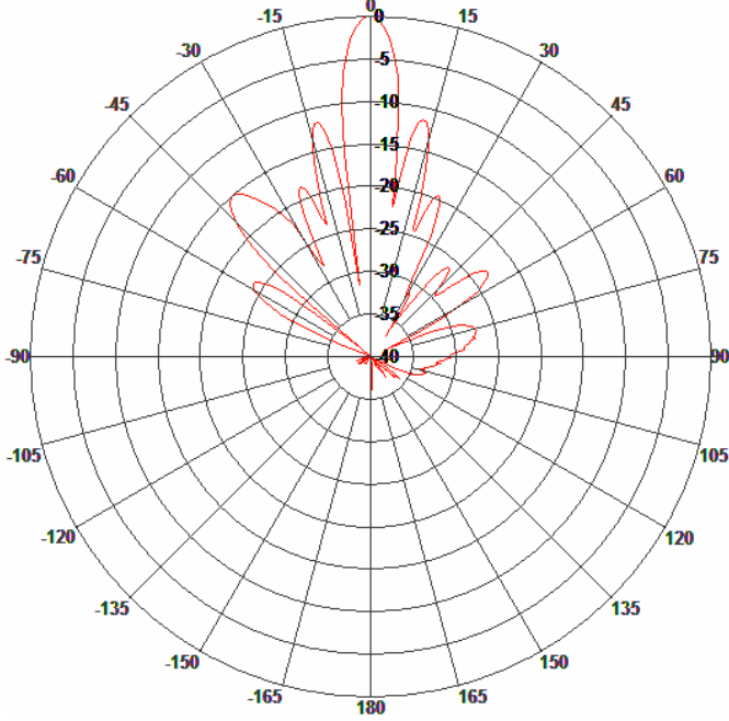
E-Plane Pattern
