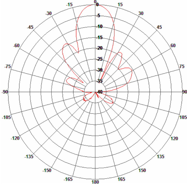
Azimuth Pattern E-Plane Pattern
