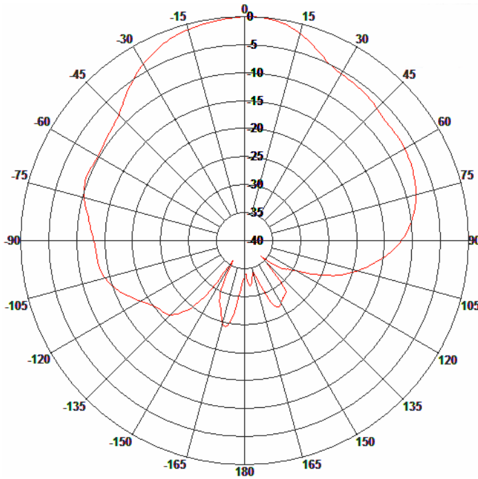
E-Plane Pattern
