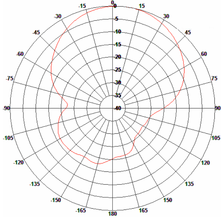
E-Plane Pattern
