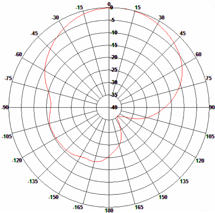
E-Plane Pattern
