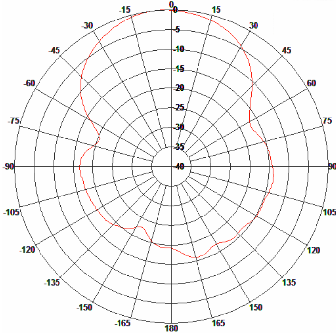
E-Plane Pattern
