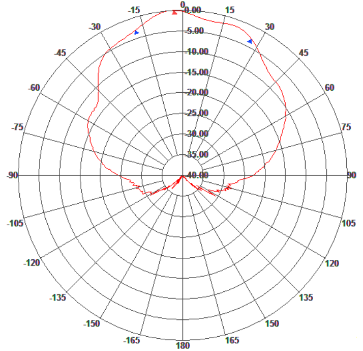
Elevation Patterns
