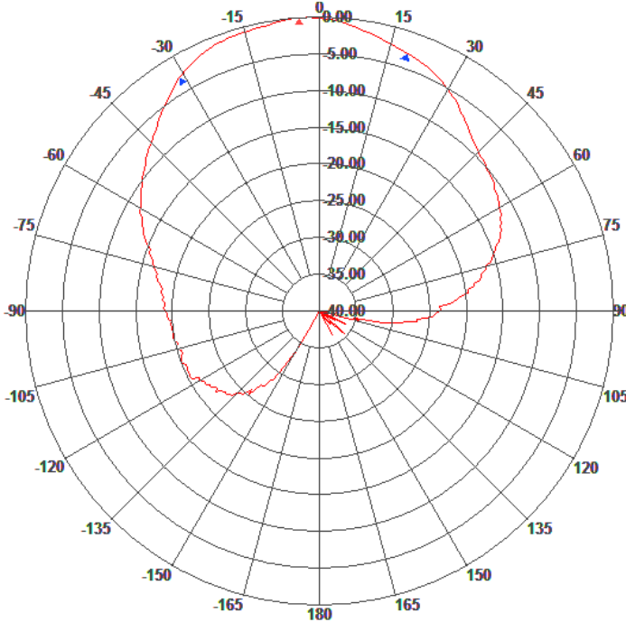
Azimuth Patterns
