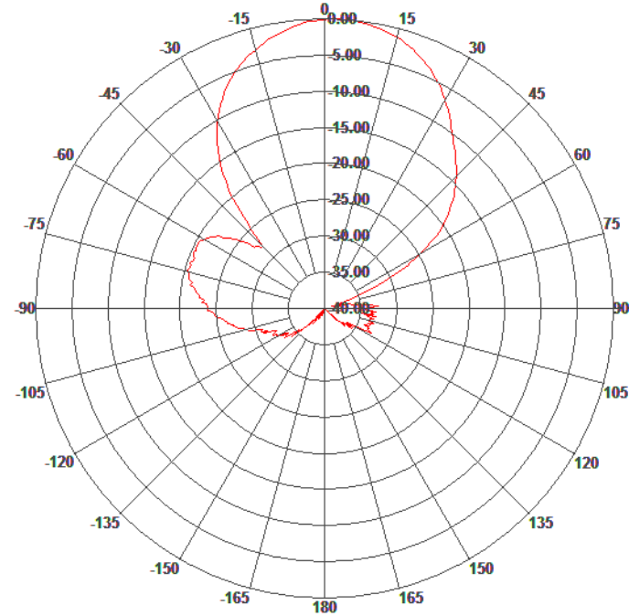
Azimuth Pattern
