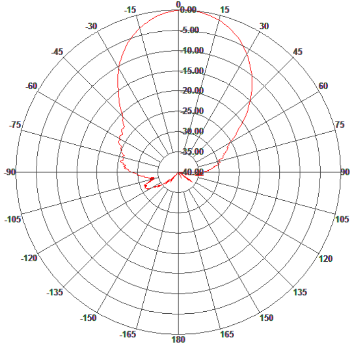
Elevation Pattern
