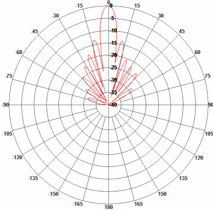
E-Plane Pattern
