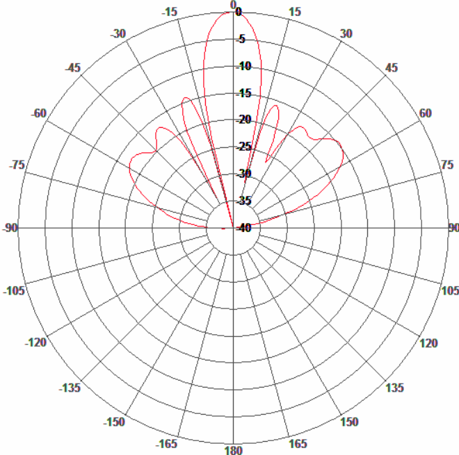
E-Plane Pattern
