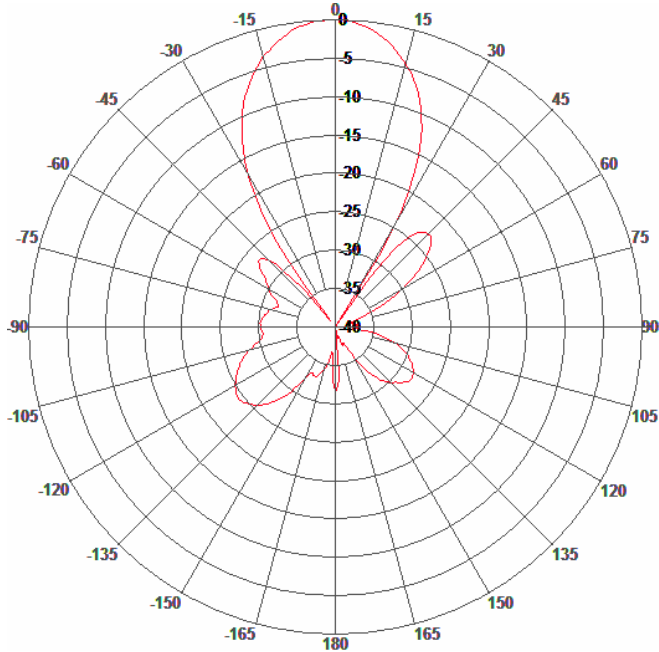
E-Plane Pattern
