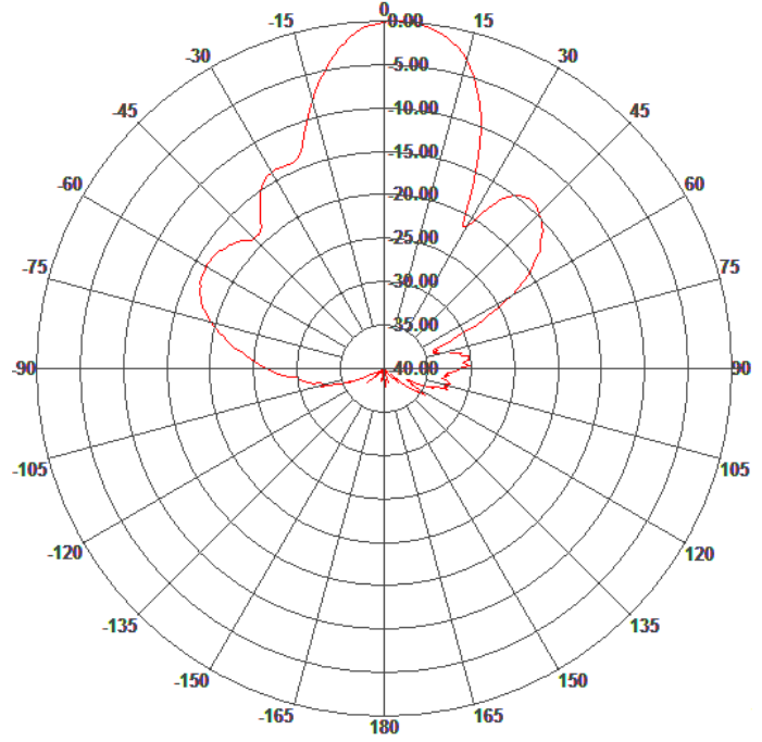
Elevation Pattern
