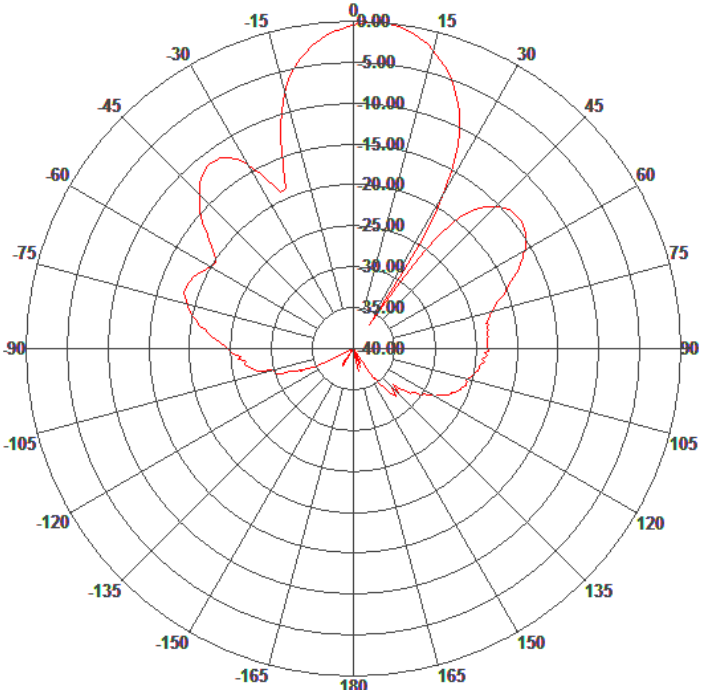
Elevation Pattern
