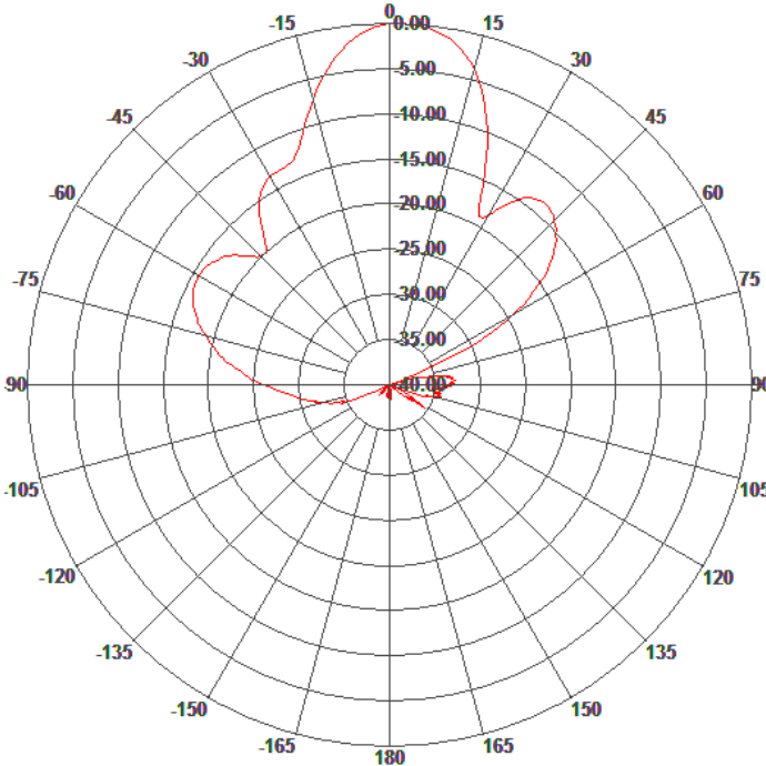
Azimuth Pattern
