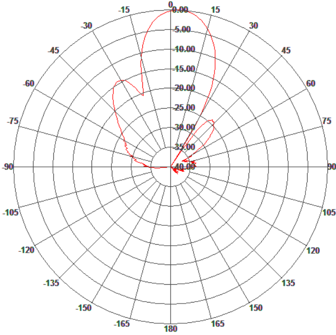
Azimuth Pattern
