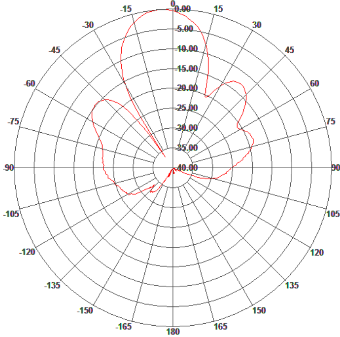
Azimuth Pattern
