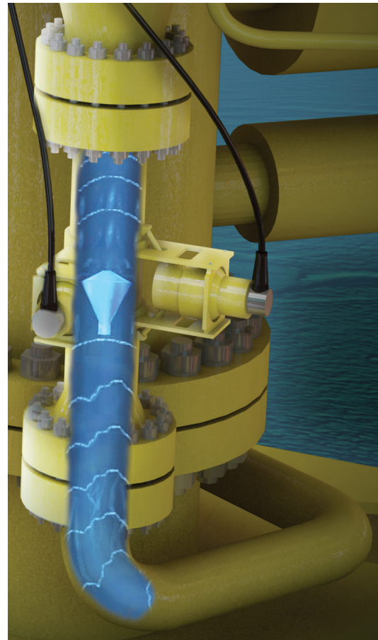
Figure 2: V-Cone Flattening Disturbed Flow Profile
