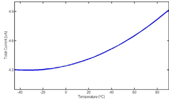
Supply Current over Temperature (No Load)
