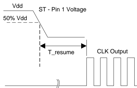
Figure 6. Resume Timing [4, 5]
