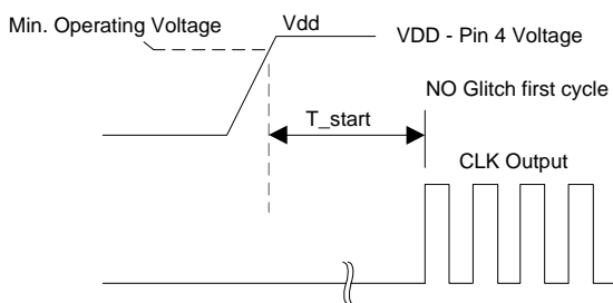
Figure 5. Startup Timing [4, 5]
