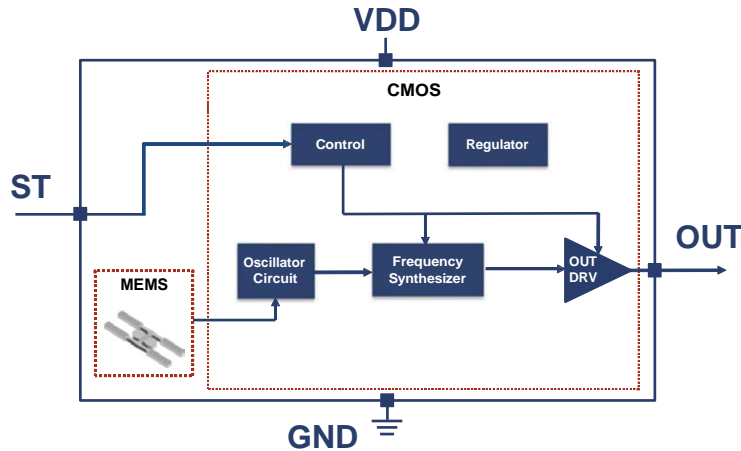
Figure 2. SiT8021 Block Diagram
