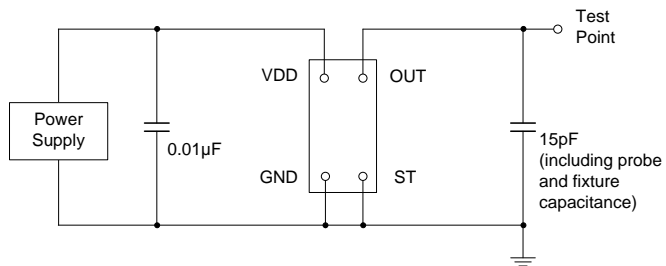
Figure 3. Test Circuit
