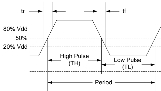
Figure 4. Waveform [3]
