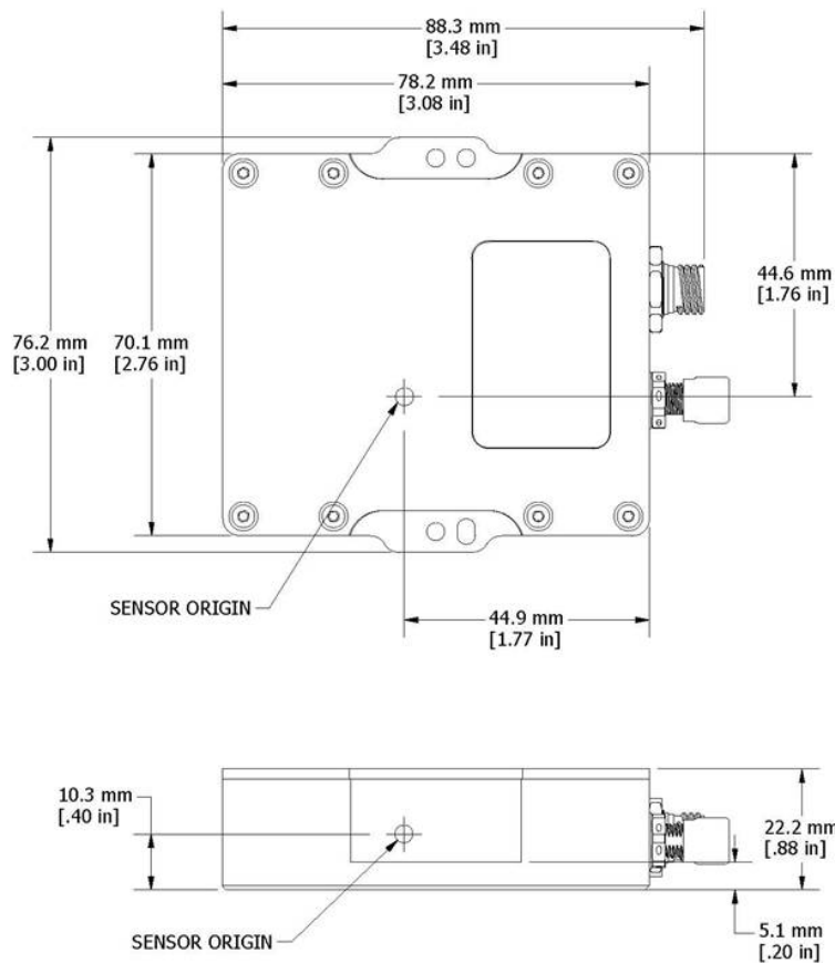
Figure 41 - 3DM-RQ1™ Sensor Origin
