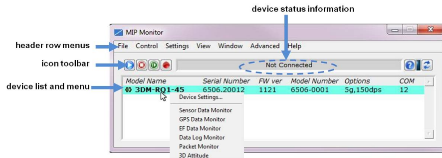
Figure 6 - Main Window
