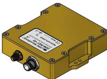
Figure 1 - 3DM-RQ1-45™ Sensor
