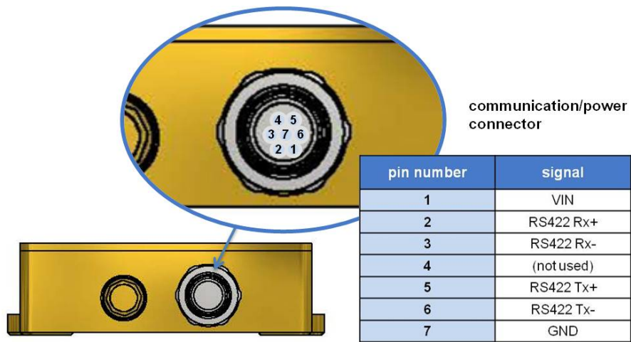
Figure 36 - Connector Wiring
