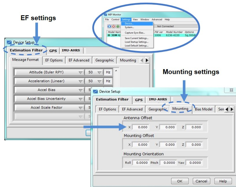
Figure 29 - Antenna Offset
