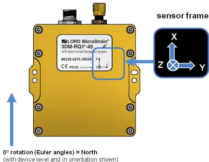
Figure 21 - Sensor Frame
