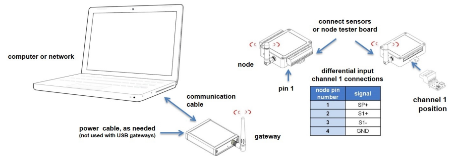
Figure 3 - System Connections
