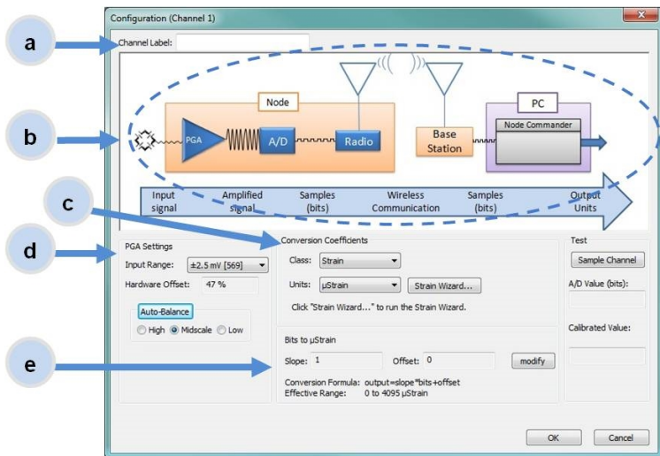
Figure 8 - Channel Setup
