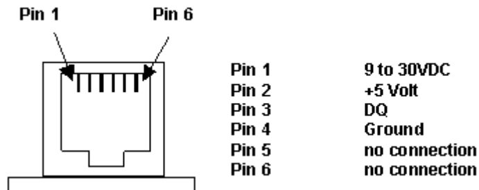
Figure 1 TEMP08 Connector Pin-out
