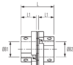
Ref. 660 for use in pairs or with floating shafts
