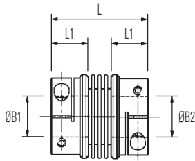
Ref. 536 Short type for precisely aligned shafts
