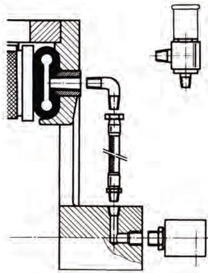
Quick Exhaust valve (QEV 40061-010/040) with silencer (SQEV 40061-510/540)
