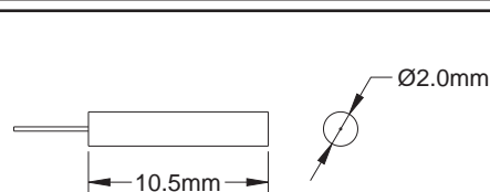
Figure 11: 2.0mm Ceramic Ferrule
