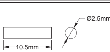
Figure 12: 2.5mm Ceramic Ferrule
