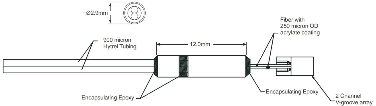
Figure 7: Two Channel V-Groove Assembly with Hermetic Patchcord
