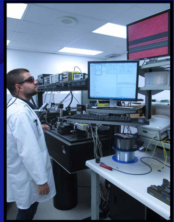
Laser Conditioning/Cleaving
