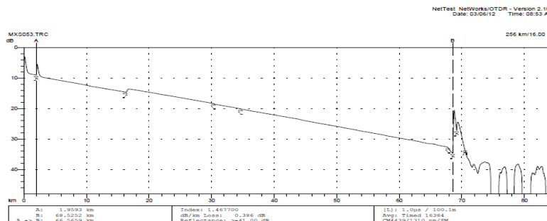
Figure 6. OTDR result on the Fiber under test
