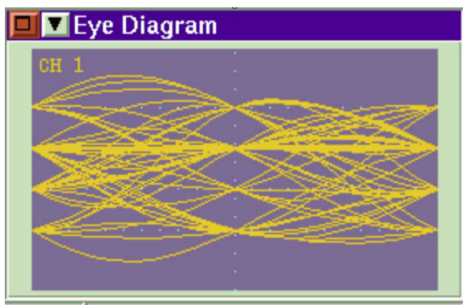
Figure 4.0 - The P25 Eye Diagram
