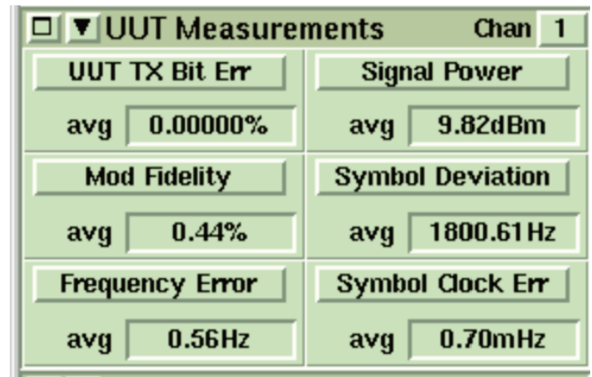
Figure 1.0 - Modulation Fidelity Measurements
