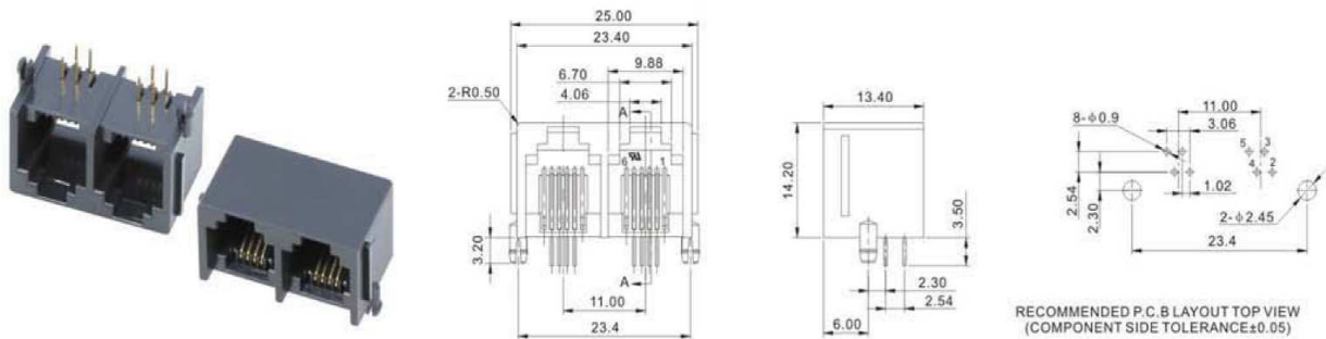
P11094-XXGXX1 5521-2R-6P4C (6C/2C)
