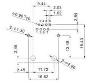
RECOMMENDED P.C.B LAYOUT TOP VIEW (COMPONENT SIDE TOLERANCE±0.05)
