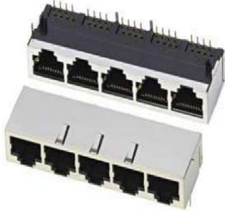
P41402-00GXX1 5921-S-BK3-A-1X5-8C(4C)-II
