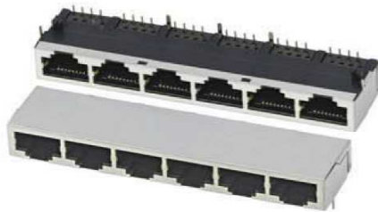
P41132-XXGXX1 5921-S-A-1X6-8C(4C)-III
