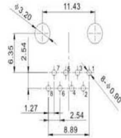
RECOMMENDED P.C.B LAYOUT TOP VIEW (COMPONENT SIDE TOLERANCE±0.05)
