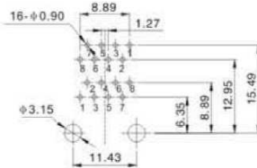
RECOMMENDED P.C.B LAYOUT TOP VIEW (COMPONENT SIDE TOLERANCE±0.05)
