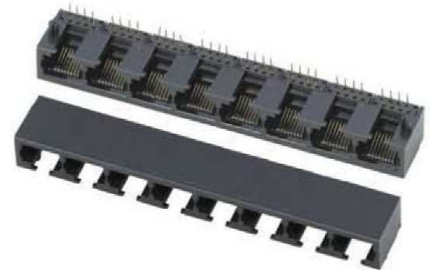
P41034-00GXX1 5622-1X8-8C(4C)
