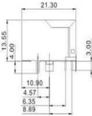
RECOMMENDED P.C.B LAYOUT TOP VIEW (COMPONENT SIDE TOLERANCE±0.05)
