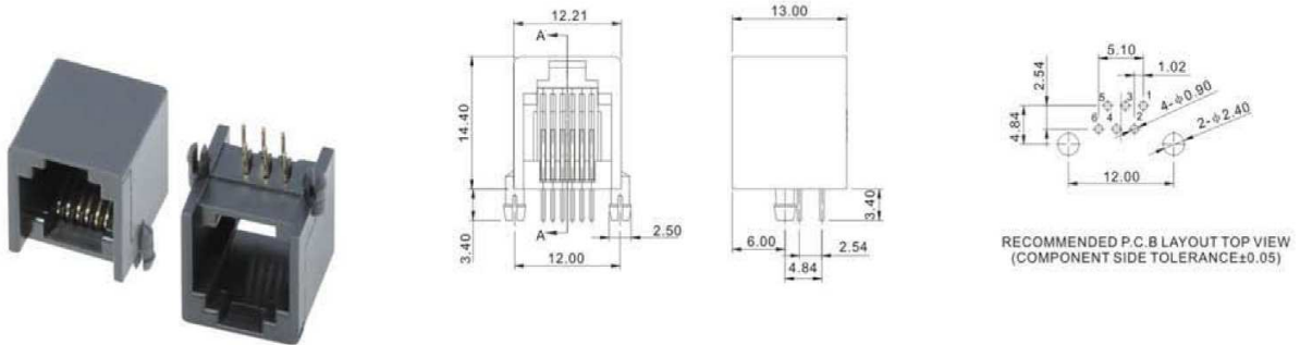
P11098-XXGXX1 5521-1-6P6C(4C/2C)
