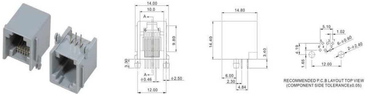
P11099-XXGXX1 5521-1R-6P6C(4C/2C)
