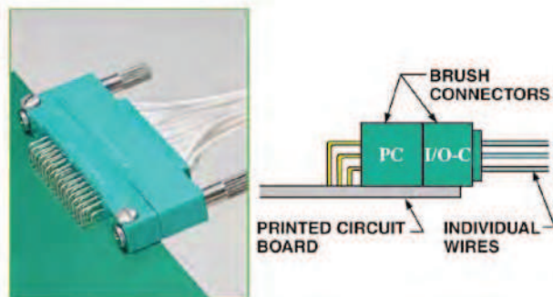
PC to I/O-C Discrete Wires to PCB
