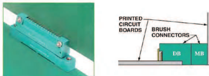
DB to MB Mating Boards at Right Angles
