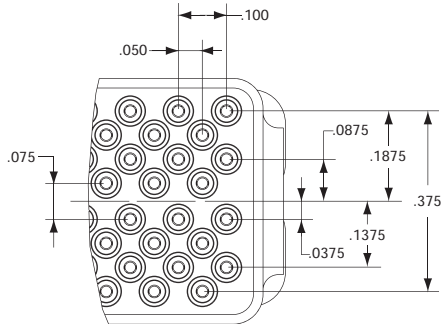
Staggered Grid for Standard Board Packages
