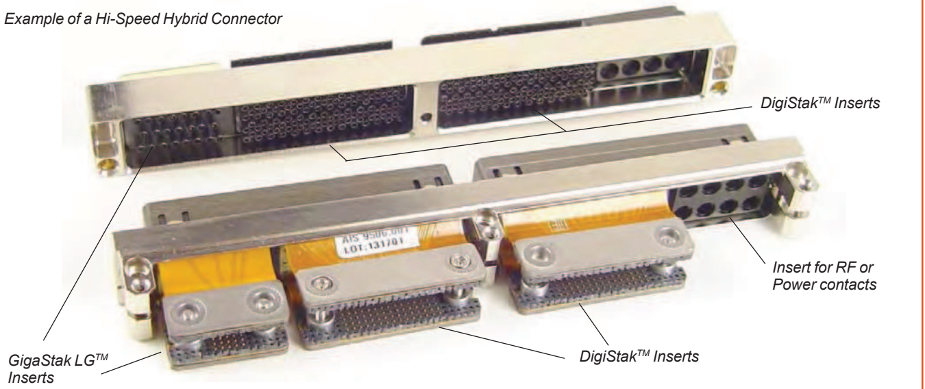
Hybrid Connector that has GigaStak-LG™ and DigiStak™ Inserts, shown on Testing Boards
