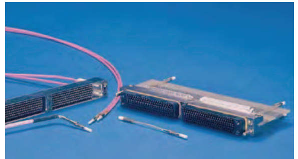
Examples of LRM connectors with fiber optic multi-mode termini in combination with brush contacts.
