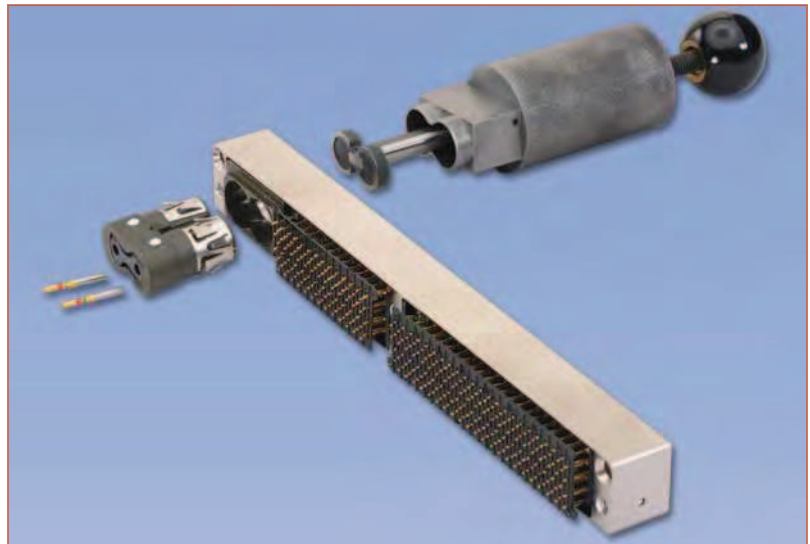
Exploded view - tool 10-507924-1 has removed power module from backplane. (size 22D contacts shown removed)
