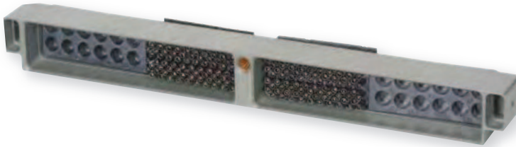
Example of a backplane connector in a 2 bay arrangement with inserts of staggered brush contacts and coax (size 12) contacts.
