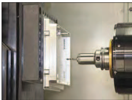
Close-up photo showing vertical machining of heatsink housings done at Amphenol.
