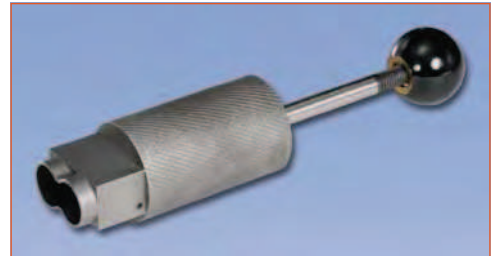
Removal tool 10-507924-1 (plunger retracted) for removing 270 VDC power modules from LRM backplanes
