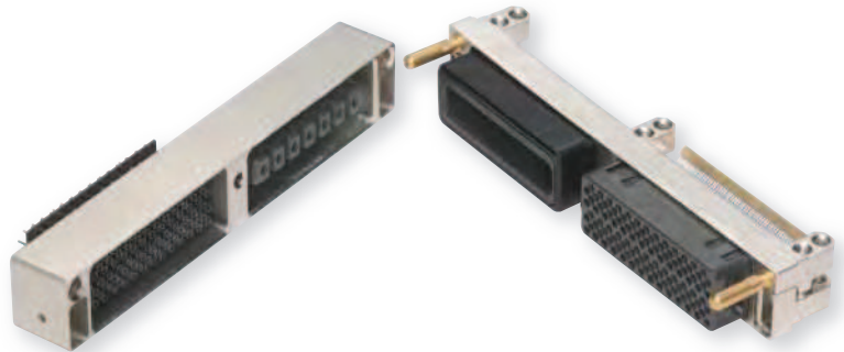
Example of a staggered grid module and backplane with 108 brush contacts and an insert for 7 size 20 crimp contacts for high voltage applications.
