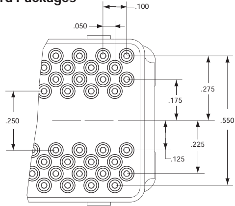
Staggered Grid Air-flow for Wider Board Packages
