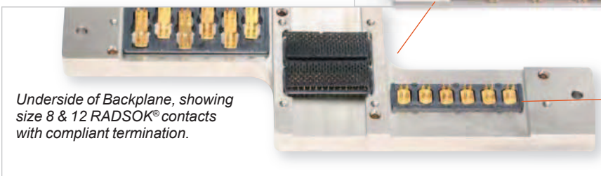
Closeup of insert with compliant pin termination power contacts.
