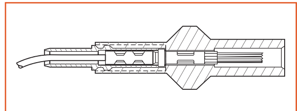
Test probe for brush contact in LRM backplane
