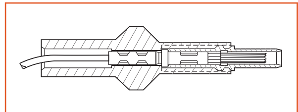
Test probe for brush contact in LRM module
