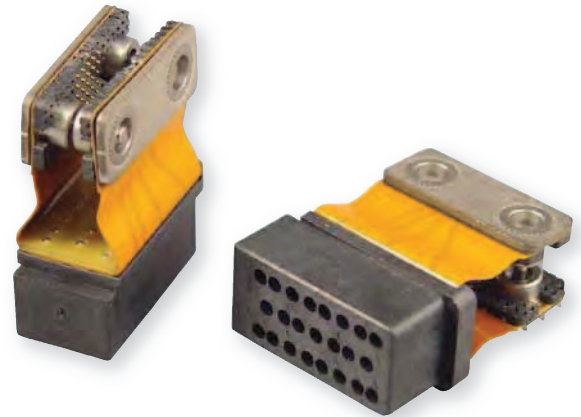
GigaStak-LG™ Inserts with 8 Hi-Speed Differential Pairs
