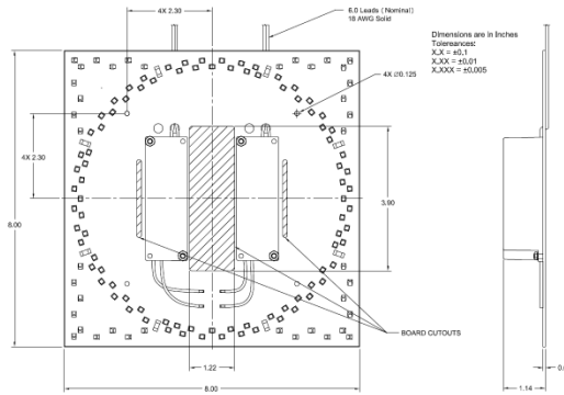
Example BEPxxMSR-xx-xx-2x (2) Drivers and ROUND LED Pattern
