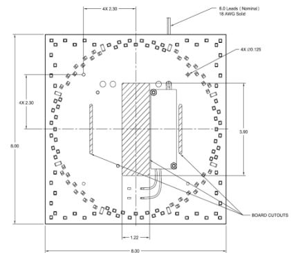
Example BEPxxMSS-xx-xx-0x (1) Driver and SQUARE LED Pattern
