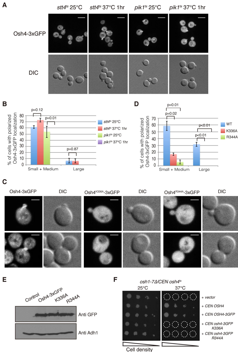
Figure 3. The polarized localization of Osh4 is dependent on PI4P
