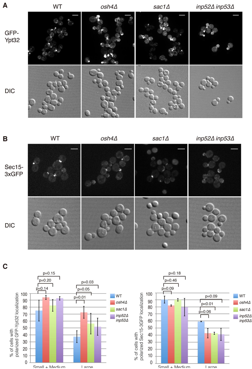
Figure 5. Osh4 regulates the distribution of Ypt32 and Sec15 in cells (A) Localization of GFP-Ypt32 in wild type cells, osh4Δ cells, sac1Δ cells and inp52Δ inp53Δ cells. Scale bar, 5 \mu m.
