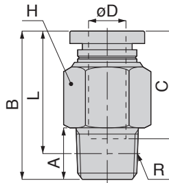
Appearance Dimension for Taper pipe thread (PT)
