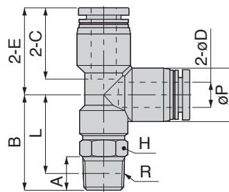
Appearance Dimension for Taper pipe thread (PT)
