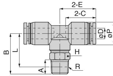
Appearance Dimension for Taper pipe thread (PT)
