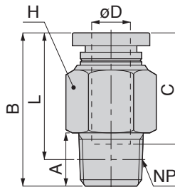
Appearance Dimension for Pipe thread general purpose (NPT)
