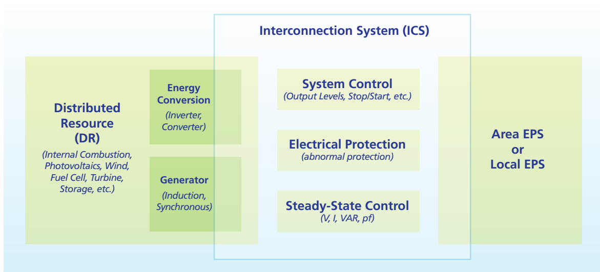
Figure 2. The characteristics of an interconnection or point of common coupling for anti-islanding prevention as identified in IEEE 1547 3 .
