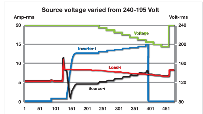
Figure 6. After voltage steps in the Transient List are programmed through the MXGUI, the resulting current and voltage steps are easily measured during the execution phase.
