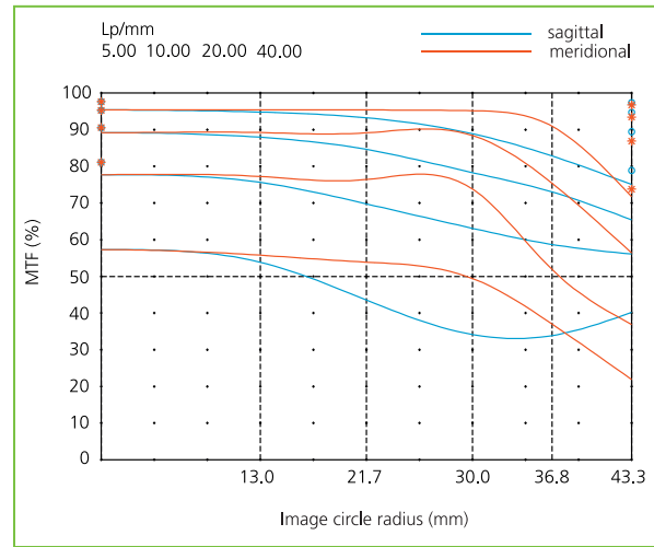
MTF of Apo-Rodagon-D 4.5/75 2x @ \beta' = -0.5 and f-stop = 5.6
