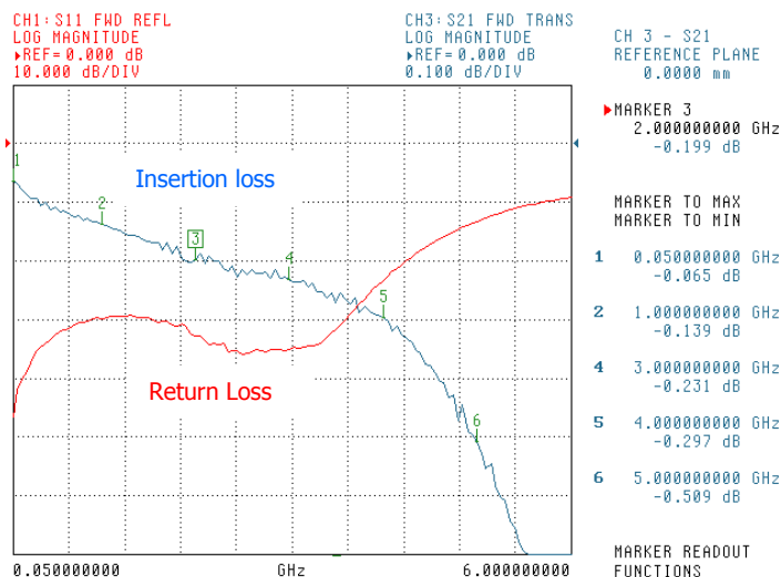
Test Board Insertion Loss
