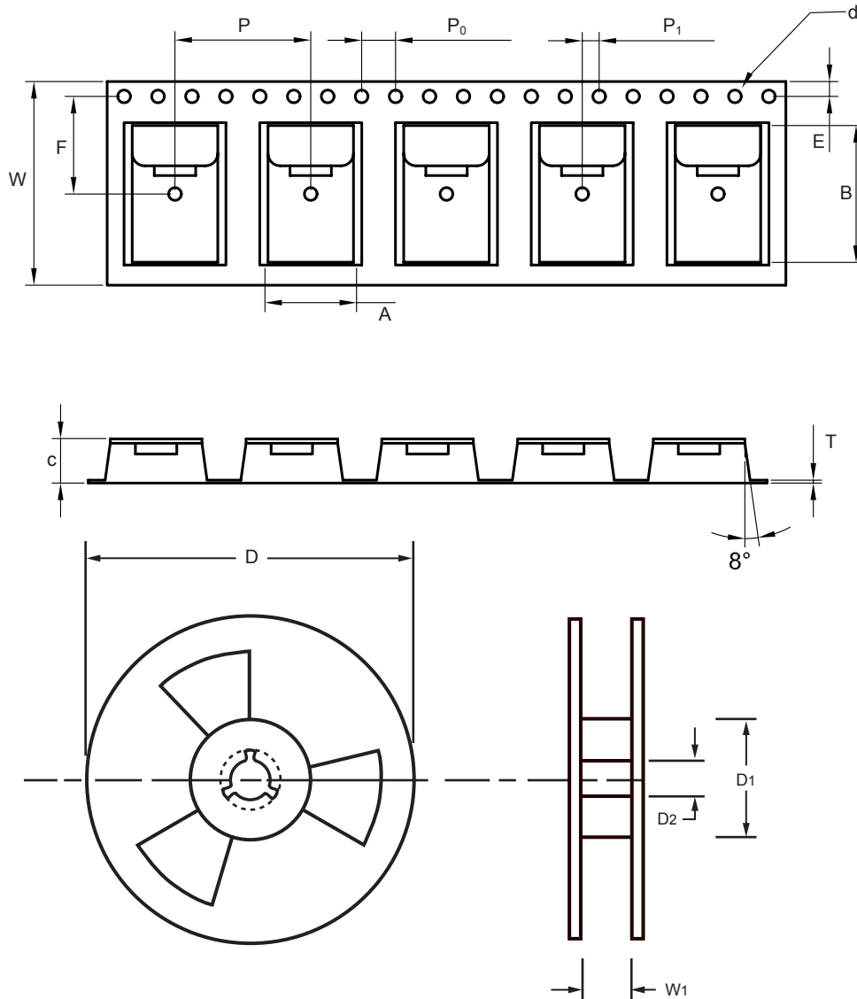
Fig.: Configuration of DIP REEL TAPING
