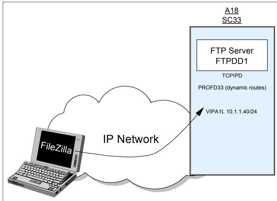
Figure 17-3 Workstation client FTP to z/OS FTP: No security
