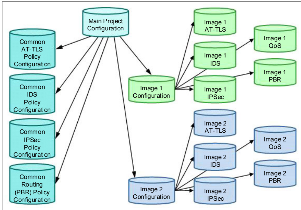
Figure 5-1 Hierarchy of PAGENT configuration files
