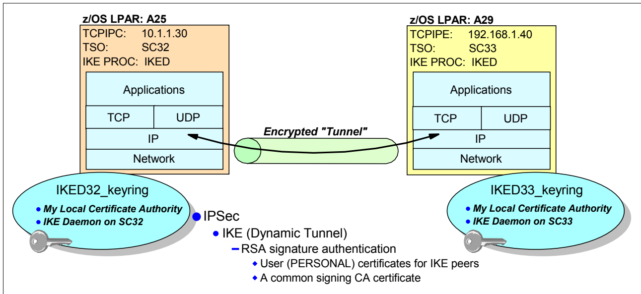
Figure 8-37 VPN tunnel between TCPIP on SC32 and TCPIPE on SC33 using RSA mode
