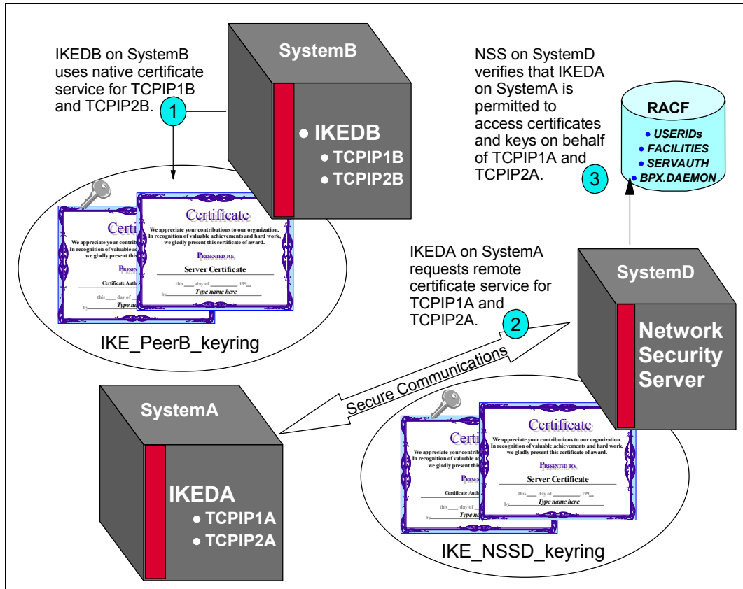
Figure 9-2 Overview of Network Security Services: Certificate management
