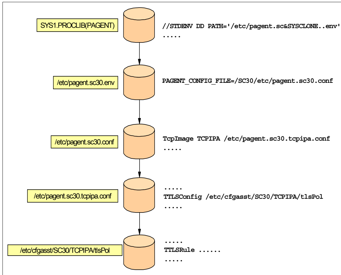
Figure 12-2 AT-TLS PAGENT configuration file relationship
