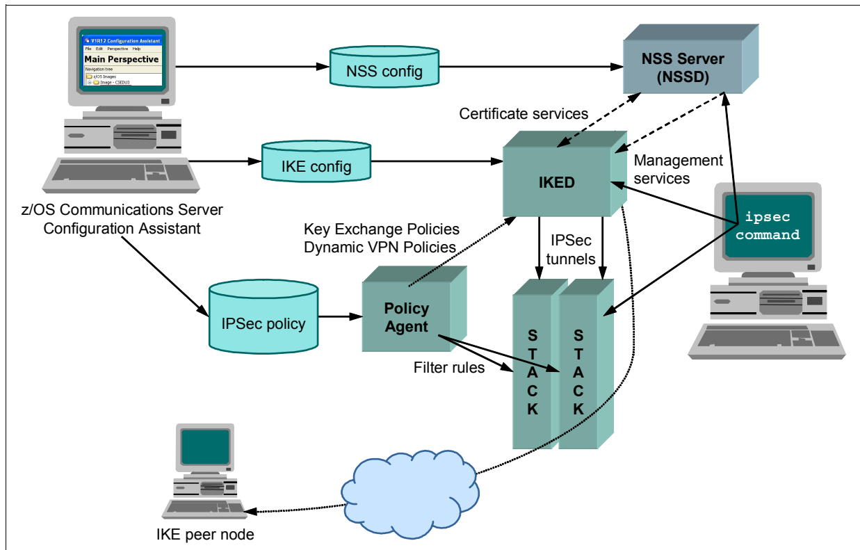
Figure 8-14 z/OS processes in IPsec
