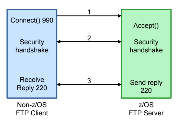
Figure 17-23 Non-z/OS FTP client implicit login with SECUREIMPLICITZOS FALSE
