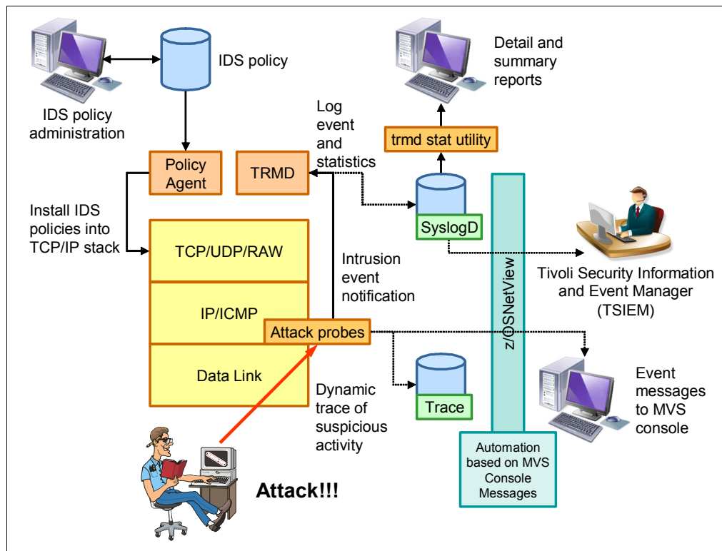
Figure 13-1 Intrusion detection services architecture
