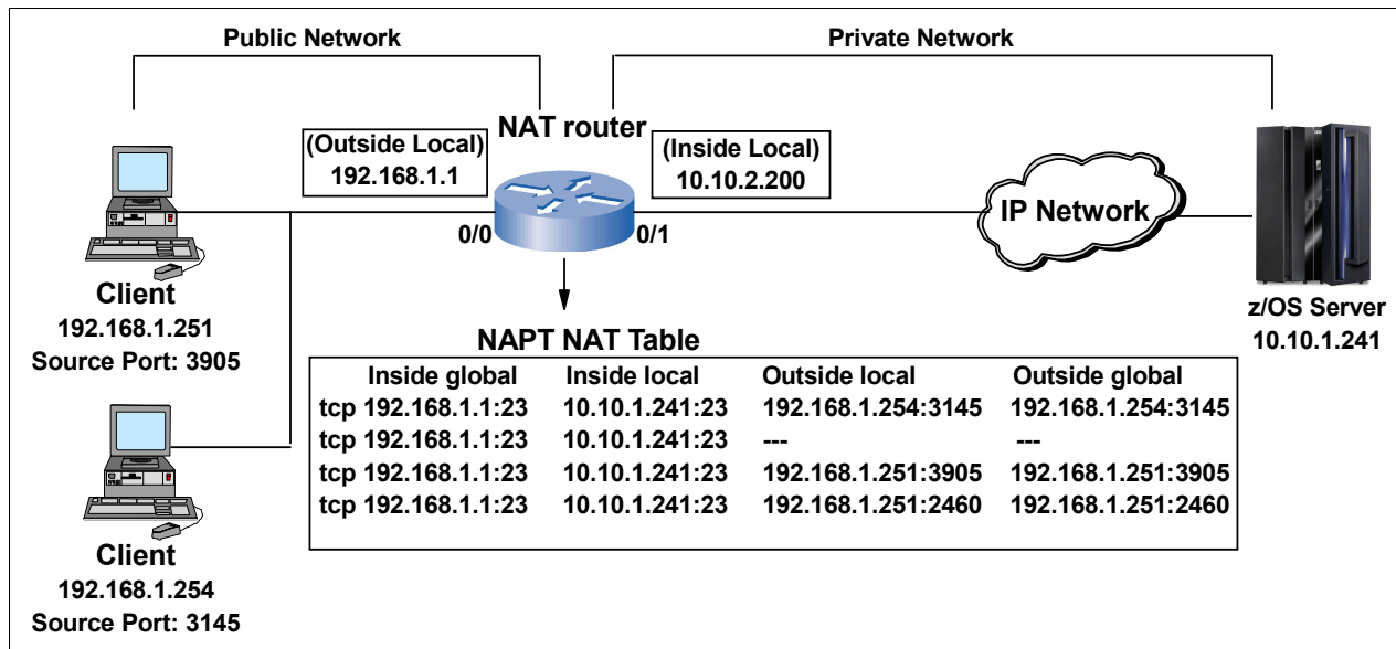
Figure 11-2 NAPT configuration example
