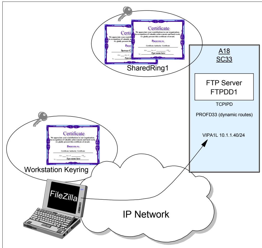
Figure 17-7 Using a Client key ring separate from the Server key ring
