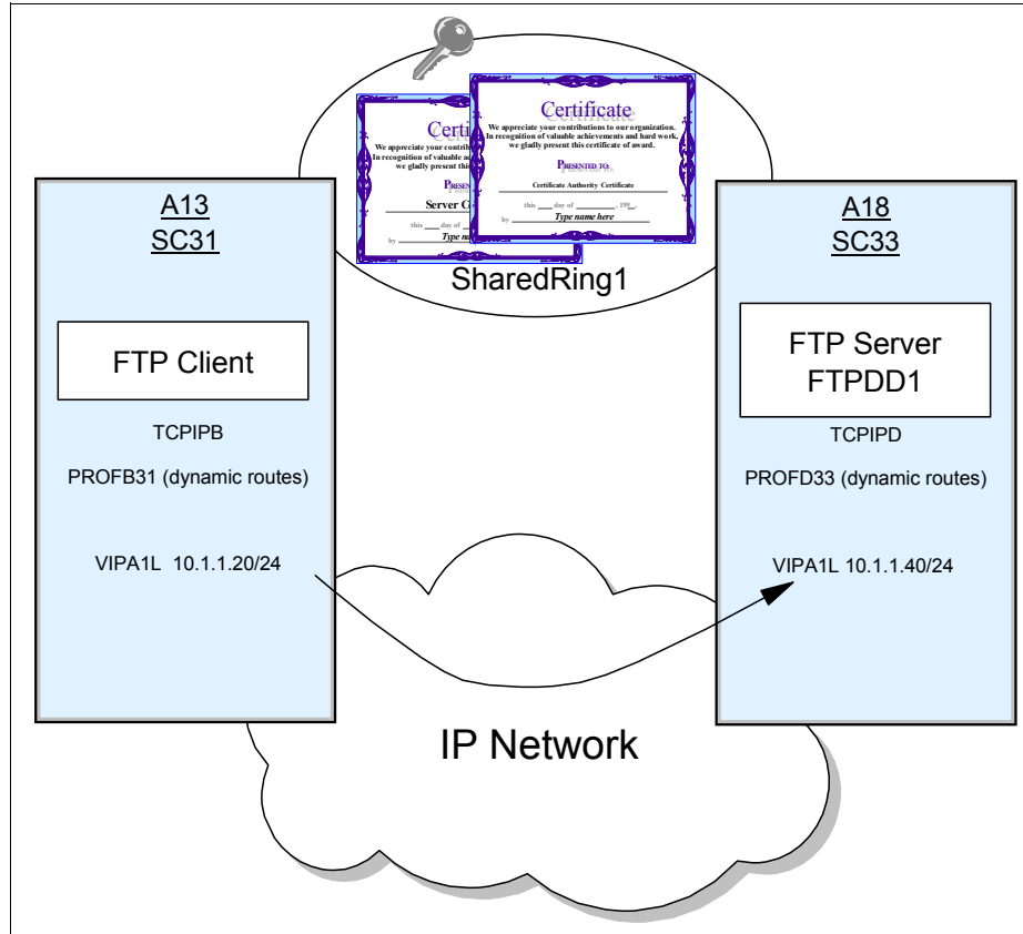
Figure 17-6 z/OS Client to FTP server: TLS Security
