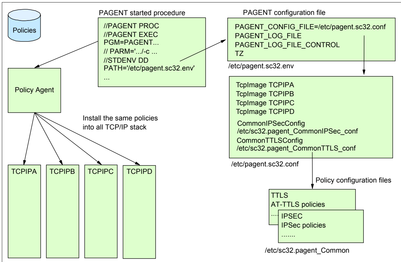
Figure 4-6 Multiple stacks, single policy definition
