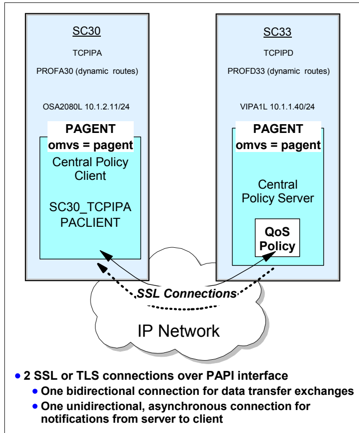
Figure 5-5 QoS policy maintained at centralized policy server and sent to policy client
