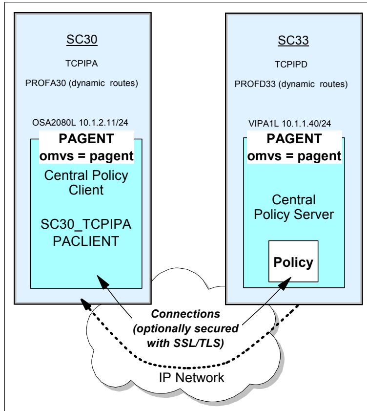
Figure 5-3 Relationship between centralized policy server and policy client
