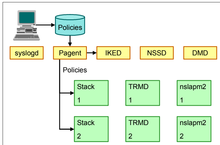
Figure 4-7 Policy infrastructure elements
