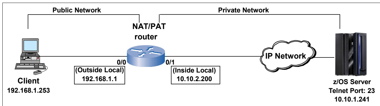
Figure 11-3 NAPT traversal test environment
