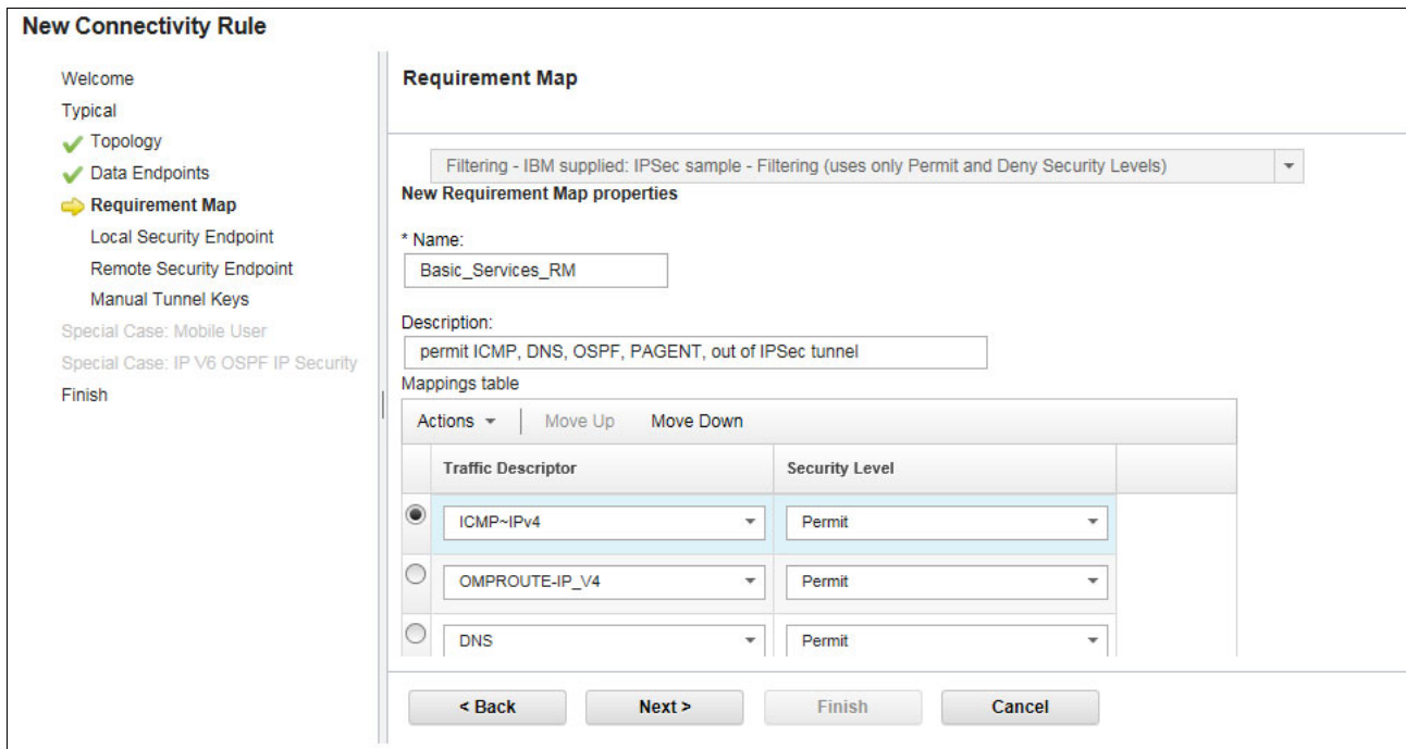
Figure 8-23 Add the BasicServices requirement map
