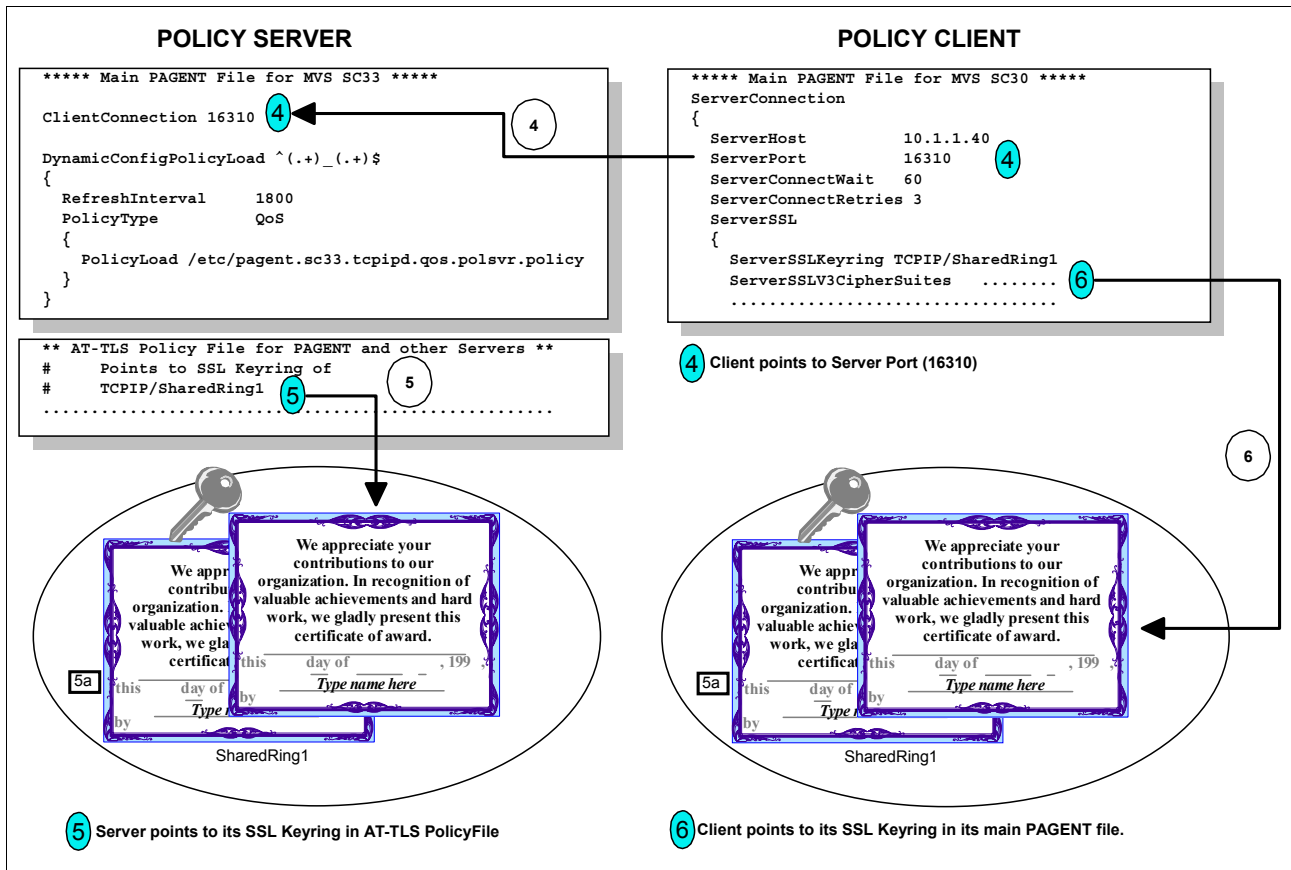
Figure 5-19 Shared key ring for the SSL connection between server and client
