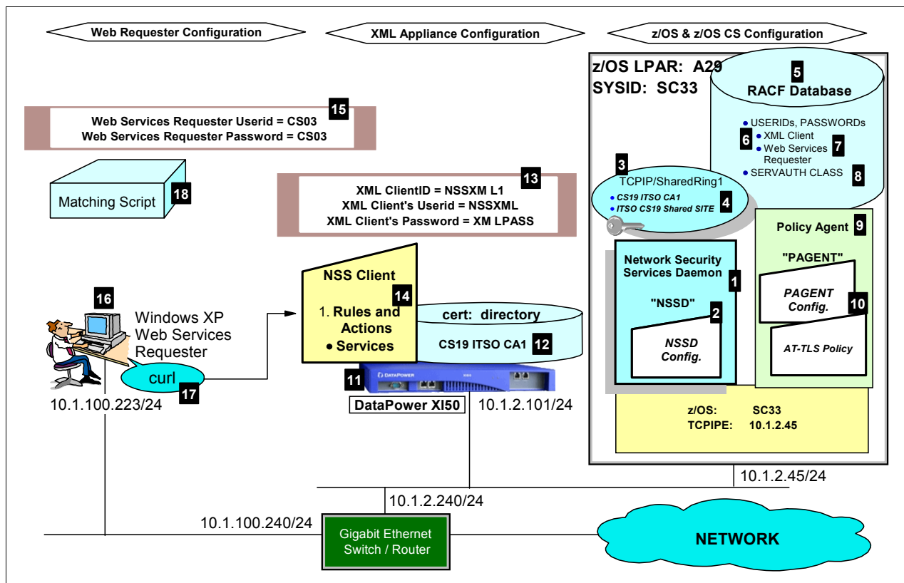
Figure 10-6 Implementation detail for the XMLAppliance Discipline
