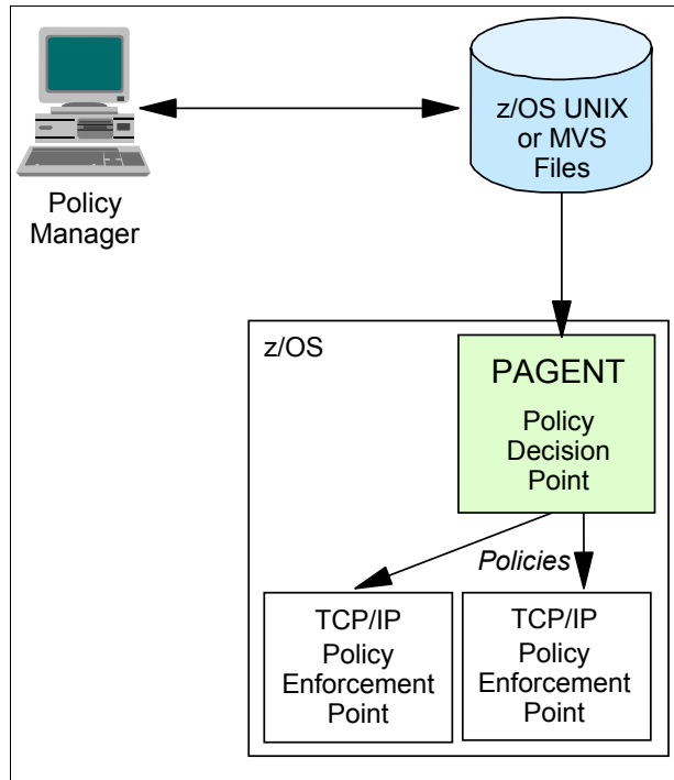
Figure 4-2 Policy system model
