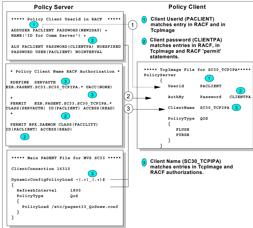
Figure 5-18 Correlation of client user ID, client password, client name at server and client
