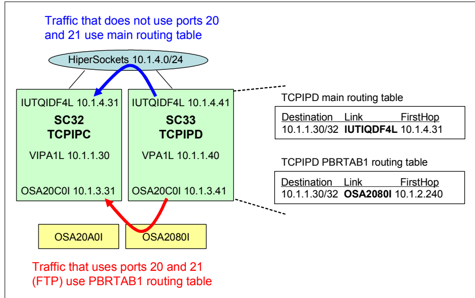
Figure 15-16 PBR using protocol and port numbers
