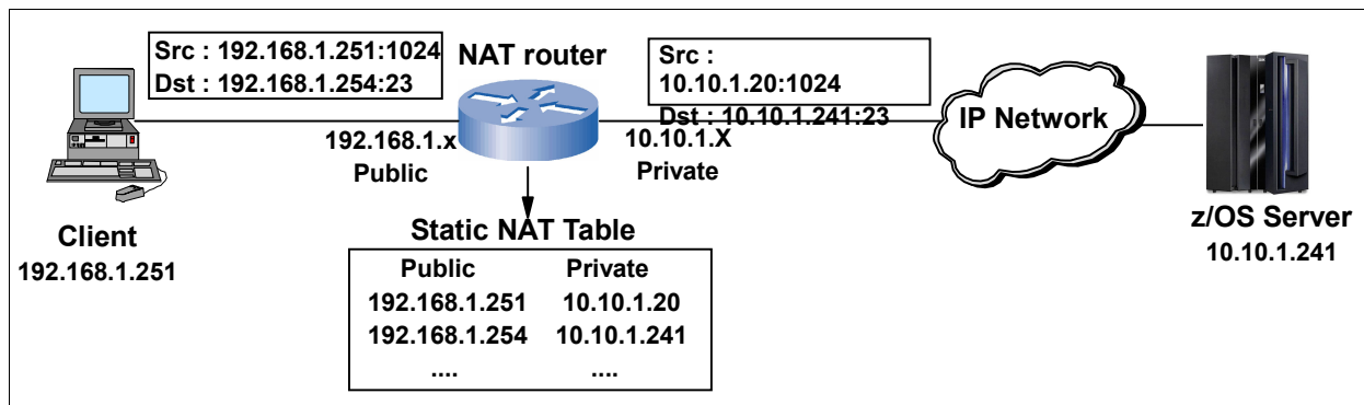
Figure 11-1 Static NAT
