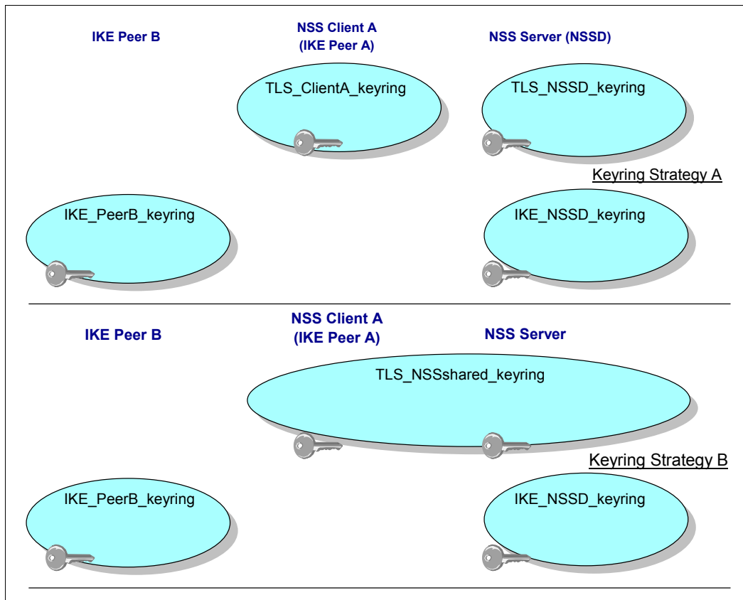
Figure 9-7 Key ring strategies for an NSS implementation
