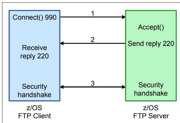
Figure 17-22 z/OS FTP client implicit login with SECUREIMPLICITZOS TRUE
