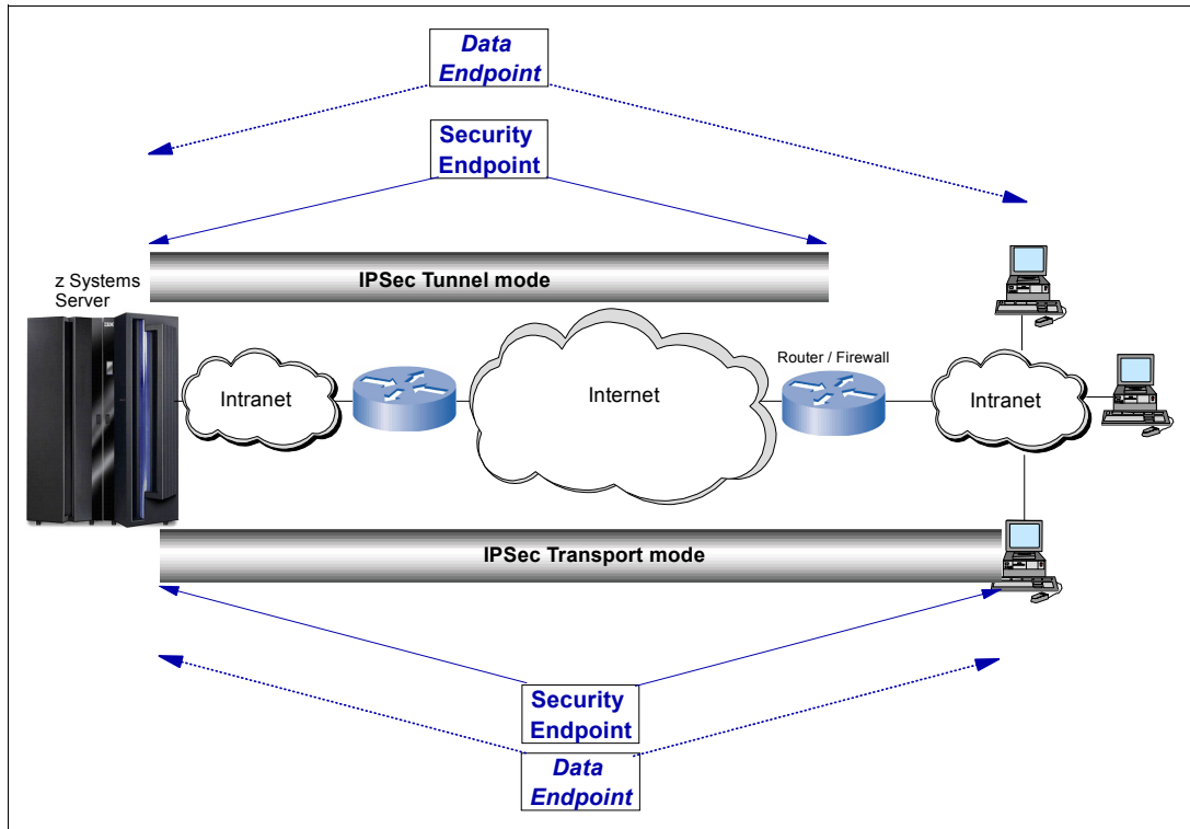
Figure 8-1 Transport mode and tunnel mode types
