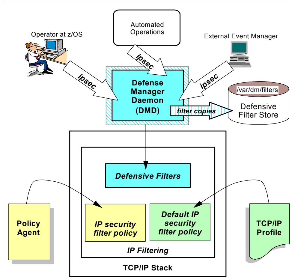
Figure 14-3 Role of defensive filtering and the Defense Manager Daemon in IP Filtering
