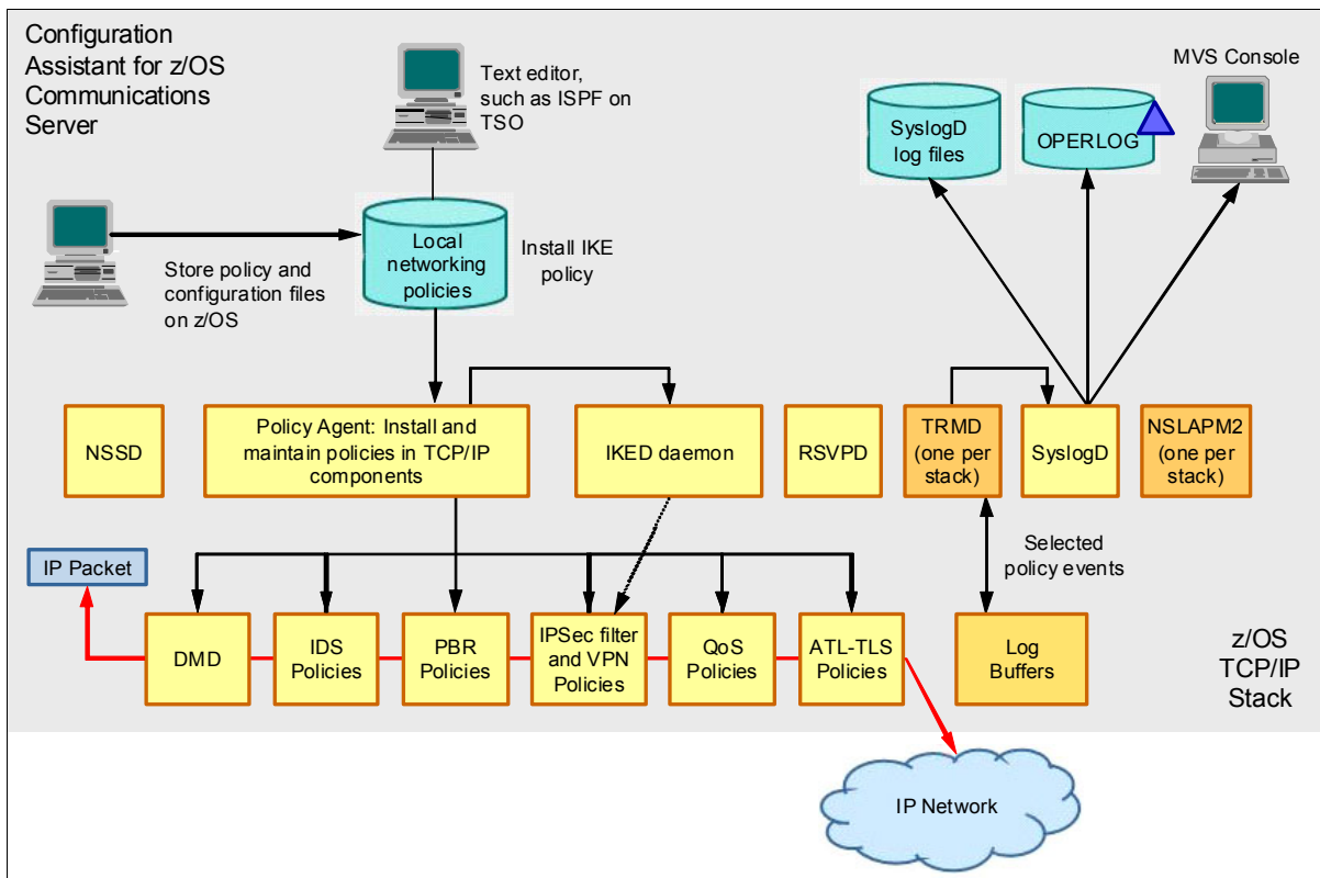
Figure 4-4 Full policy agent implementation on z/OS
