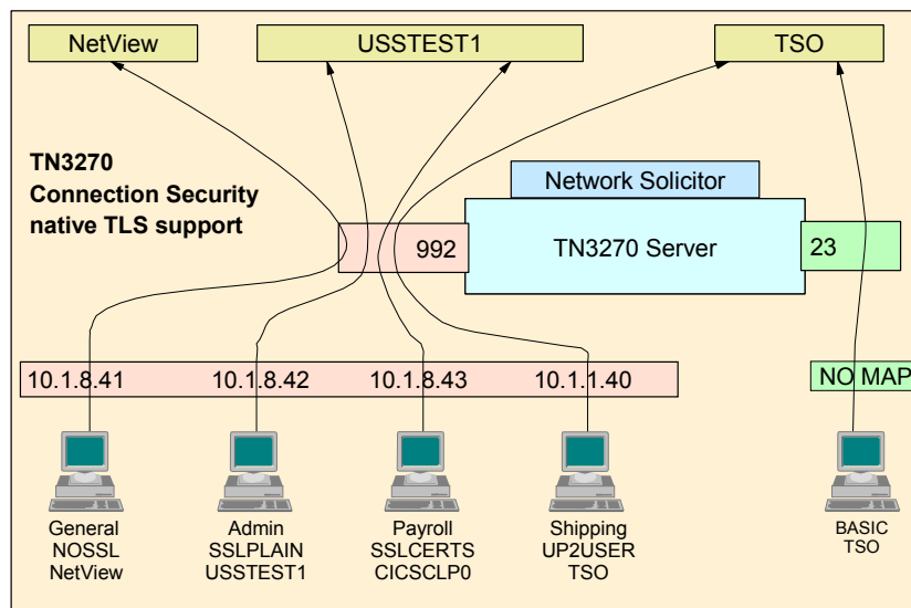
Figure B-1 Advanced native TLS configuration
