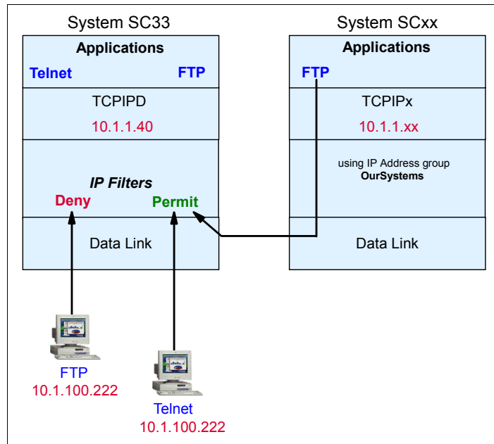
Figure 7-5 IP filtering scenario
