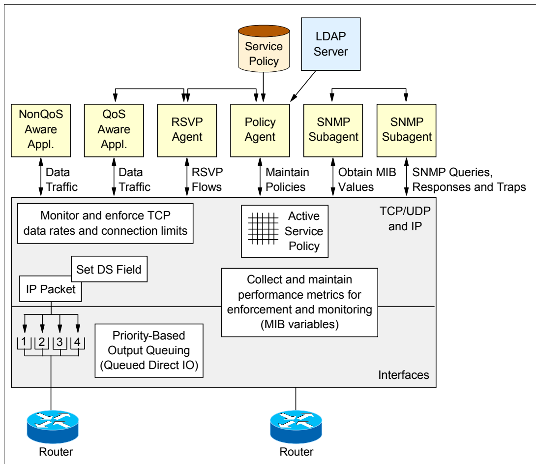
Figure 6-3 z/OS Communications Server quality of service components
