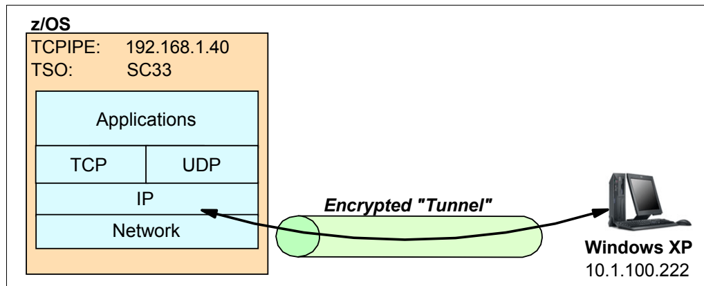
Figure C-1 VPN between z/OS and Windows
