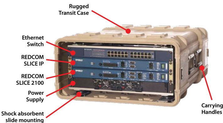
One possible TCP configuration with a REDCOM SLICE® 2100™ and SLICE® IP
