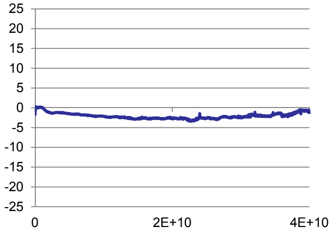
Phase Balance S31-S21
