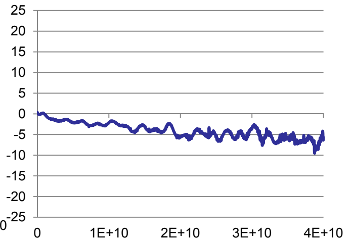
Phase Balance S41-S21
