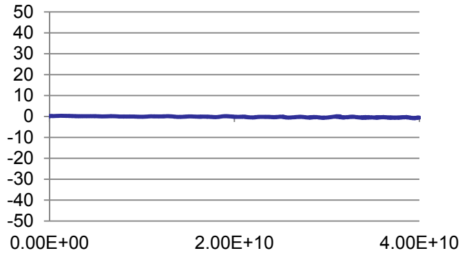
Amplitude Balance S41-S21
