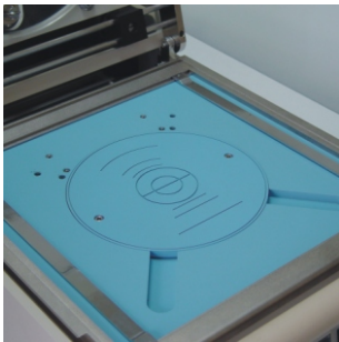
Spring – loaded floating work station to avoid wafer damage.
