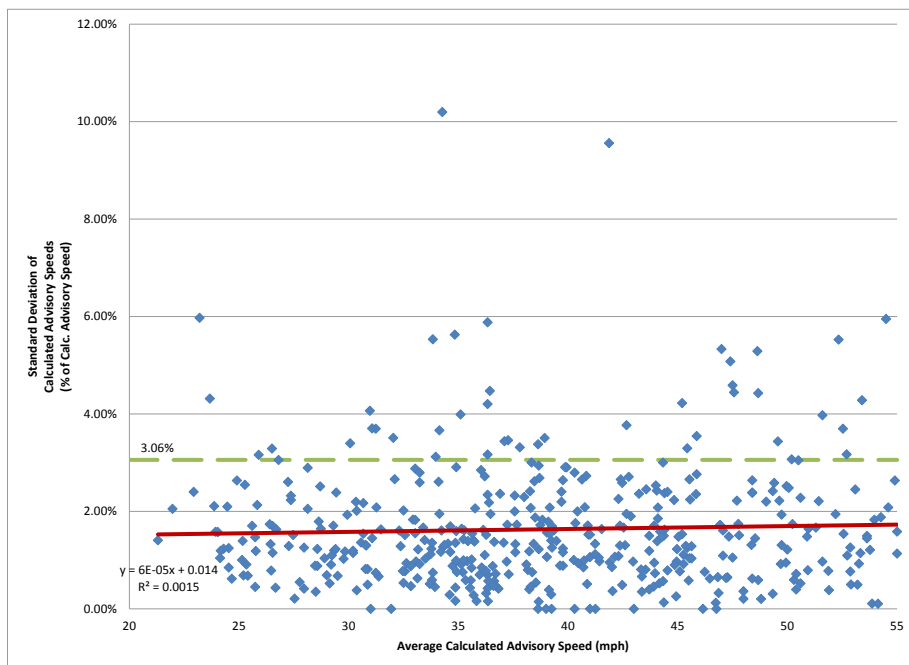
Figure 12 | Std. Dev. of Calc. Advisory Speed (%) vs. Avg. Calc. Advisory Speed
