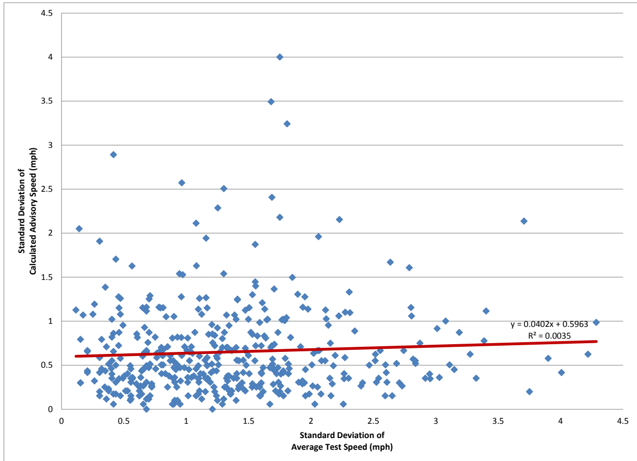
Figure 10 | Std. Dev. of Calc. Advisory Speed vs. Std. Dev. of Avg. Test Speed
