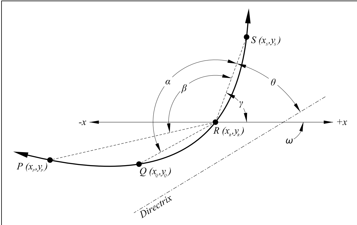
Figure 3 | Parabola through Four Points
