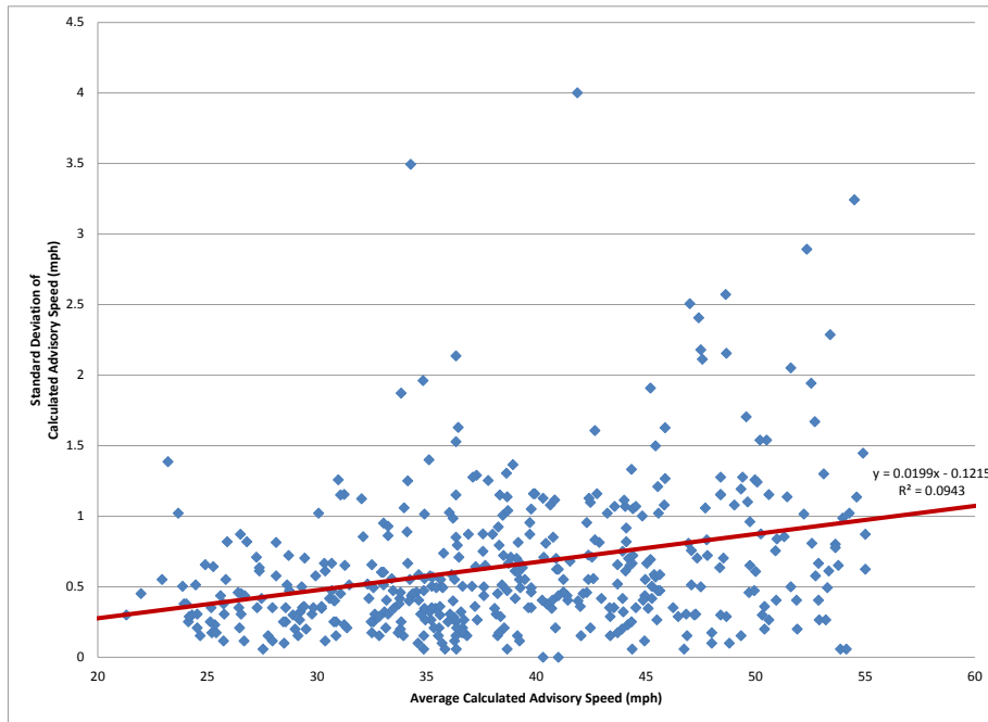
Figure 11 | Std. Dev. of Calc. Advisory Speeds vs. Average Calculated Advisory Speed
