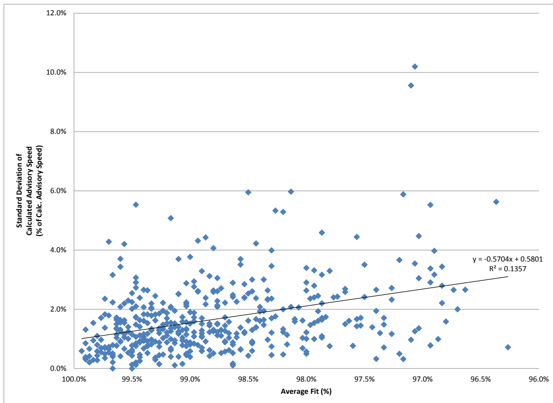
Figure 14 | Std. Deviation of Calc. Advisory Speed vs. Average Fit
