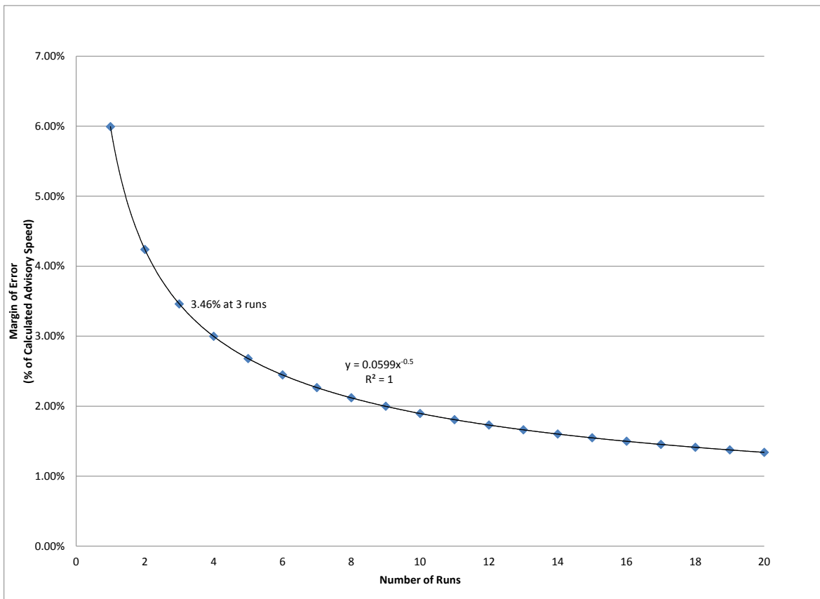
Figure 13 | Margin of Error vs. Number of Runs – 95% Confidence Interval
