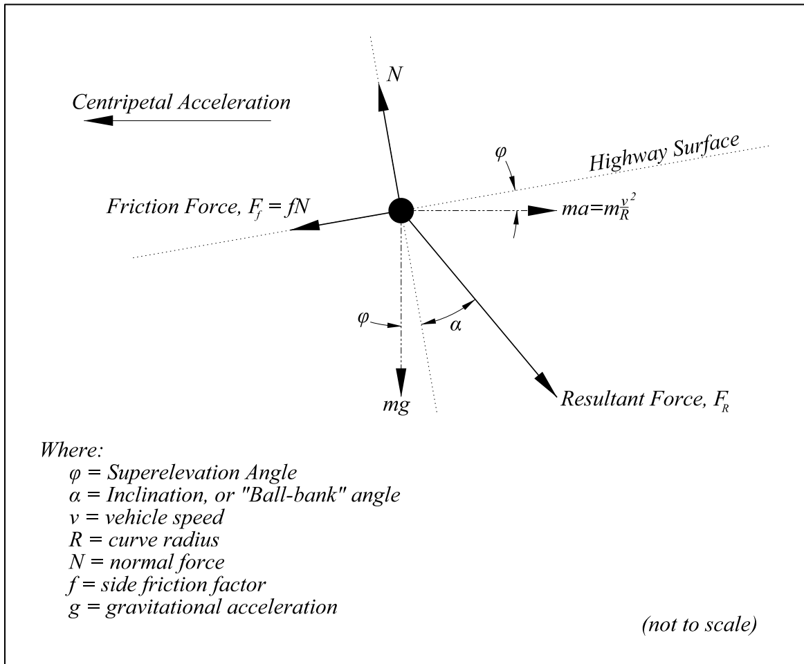
Figure 1 | Geometry of Forces Acting on Vehicle (ignoring the effects of body roll)
