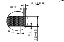
DETAIL B 5 : 1 NOT TO SCALE
