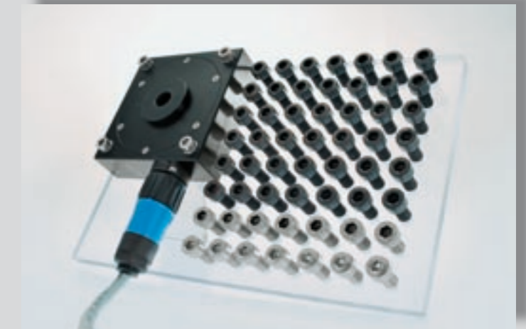
Coil for sorting test with screws of different tensile strengths
