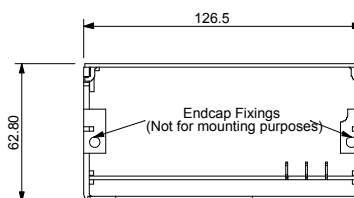
Customer Air Case (no fan)
