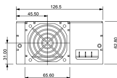
Screw & Fast-on Terminal Case
