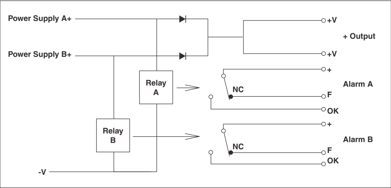
Block Diagram DLP-PU Series
