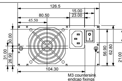
IEC-320 Connector Case
