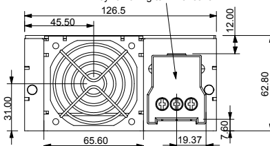
Screw & Fast-on Terminal Case
