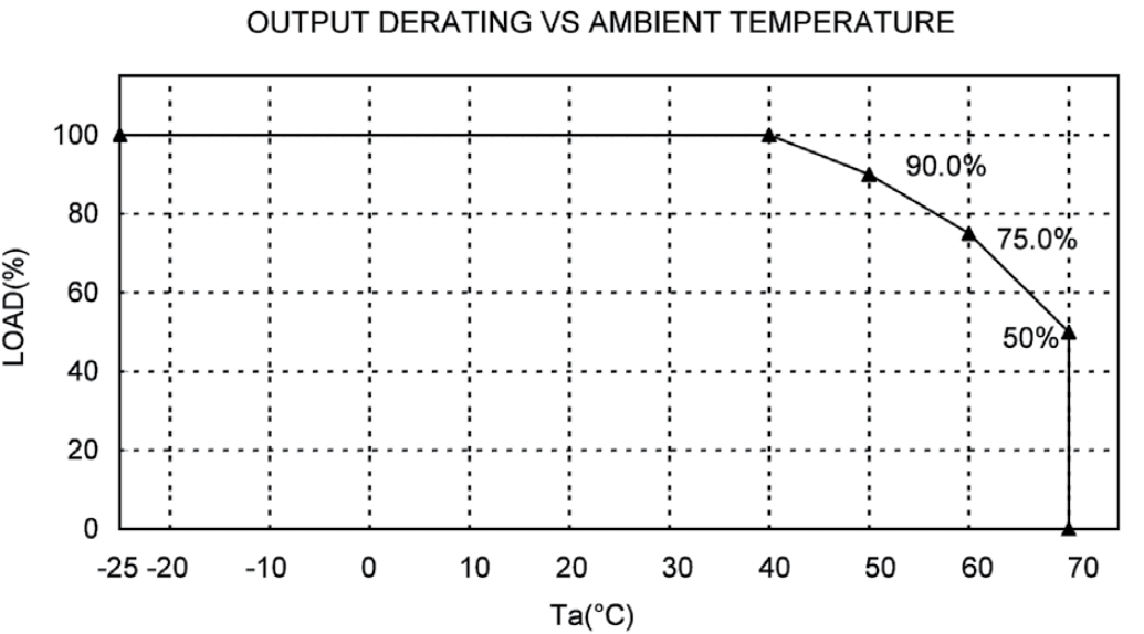
Output Derating Curve CUS250LD
