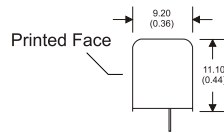
8 Pin SIL Package Nickel-Coated Copper
