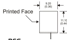
8 Pin SIL Package Non-Conductive Plastic
