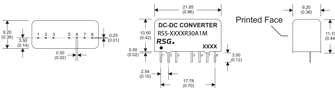
8 Pin SIL Package Nickel-Coated Copper
