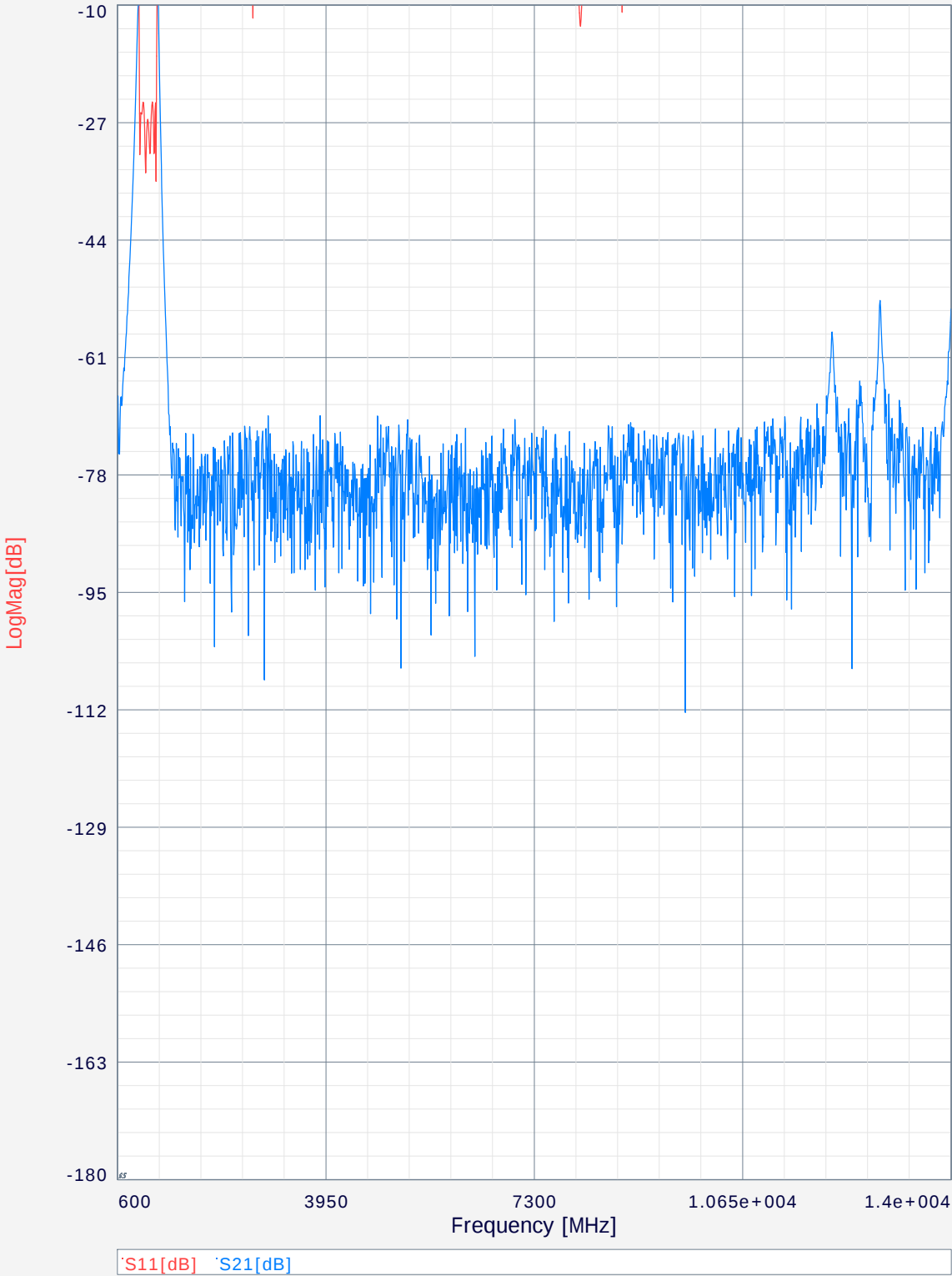
S1 91122TO14GHZ.s2p
