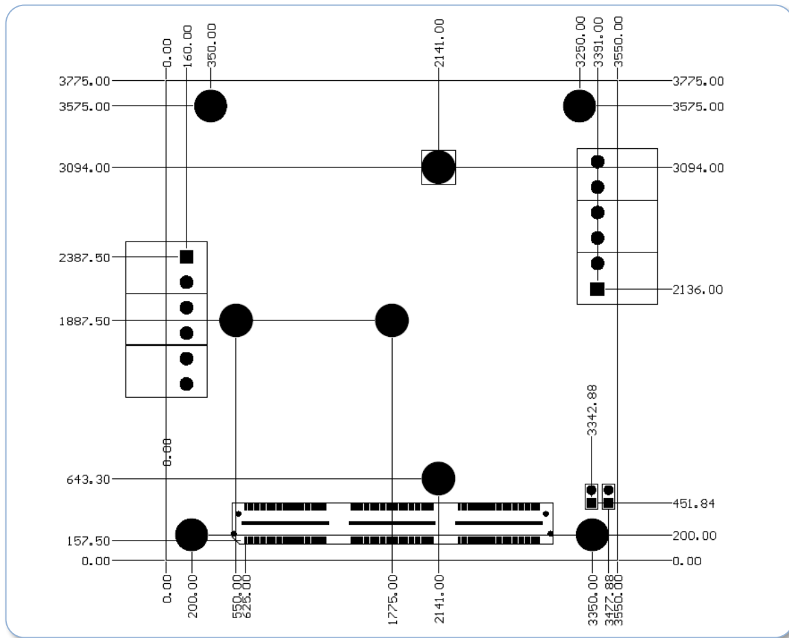
Figure 2: Board Dimensions
