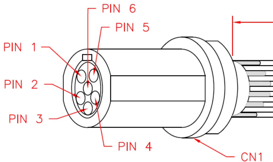
Figure 9 Power Input Connector
