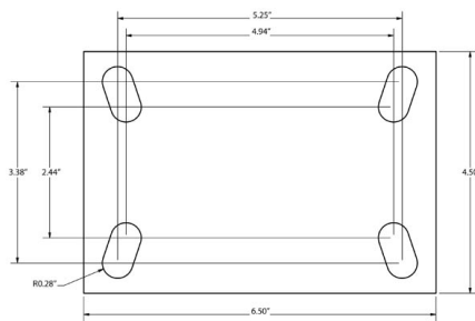
Standard Swivel Top Plate
