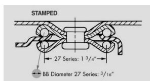
Kingpin Swivel Section
