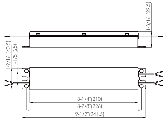
Dimensions: (inches/mm)
