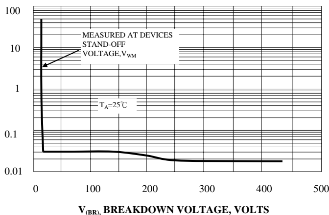
FIG. 6 - TYPICAL REVERSE LEAKAGE CHARACTERISTICS
