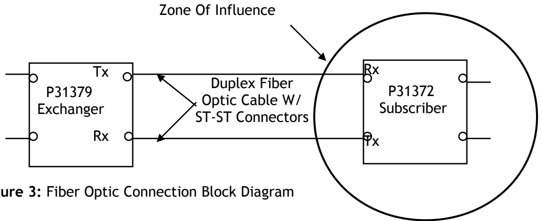
Figure 3: Fiber Optic Connection Block Diagram
