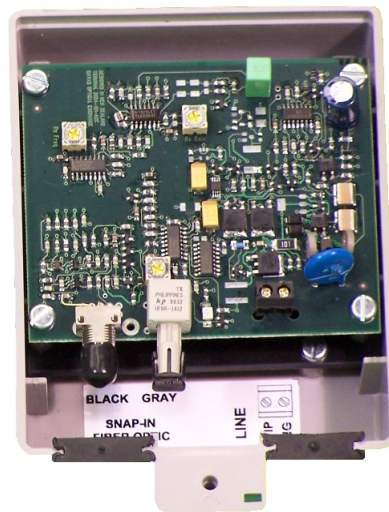
B: Top View With Cover Removed
