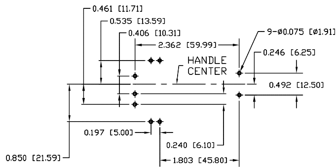
P.C. FOOT PRINT FOR TERMINAL CODE L
