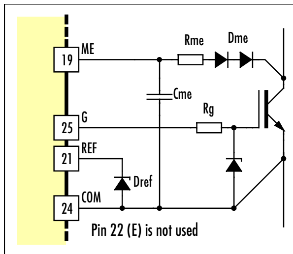
Fig. 6 Unipolar gate driving (0/+15V)
